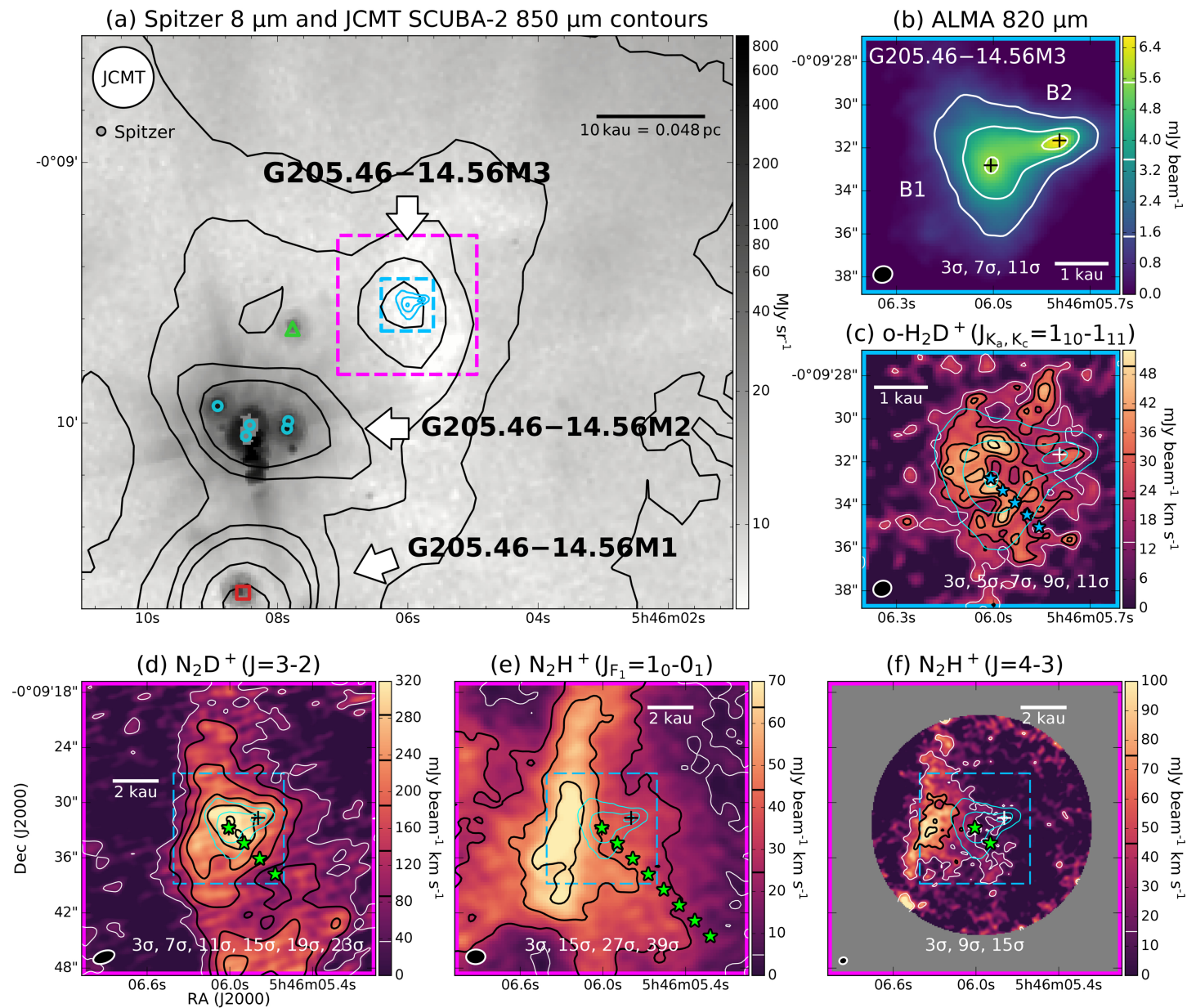
Figure 1. from Sheng-Jun Lin et al 2025 Astrophys. J. 995 doi:10.3847/1538-4357/ae0cb5 https://dx.doi.org/10.3847/1538-4357/ae0cb5 © 2025. The Author(s). Published by the American Astronomical Society.
