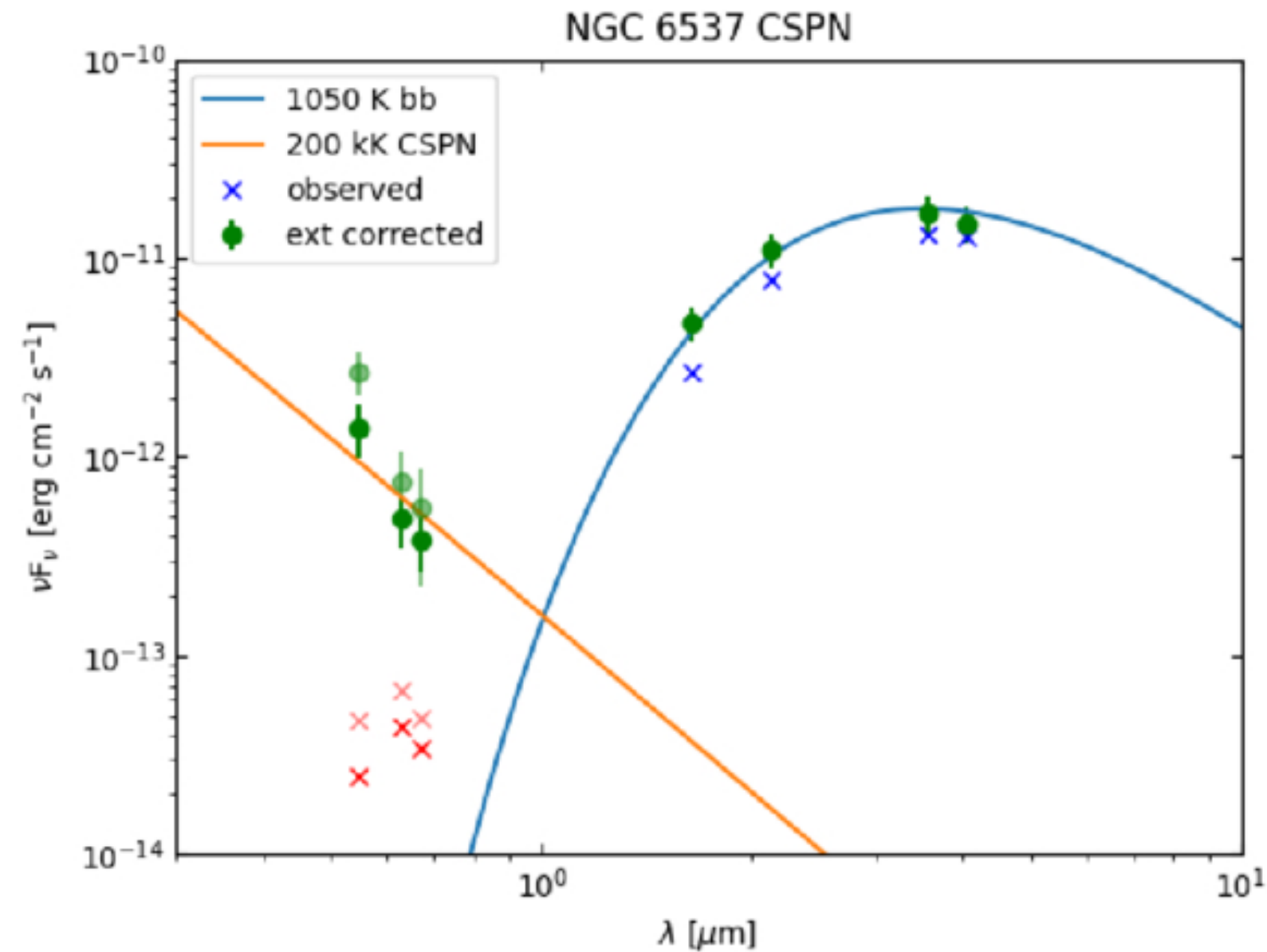
Figure 9. from Joel H. Kastner et al 2025 Astrophys. J. 993 doi:10.3847/1538-4357/ae0706 https://dx.doi.org/10.3847/1538-4357/ae0706 © 2025. The Author(s). Published by the American Astronomical Society.
