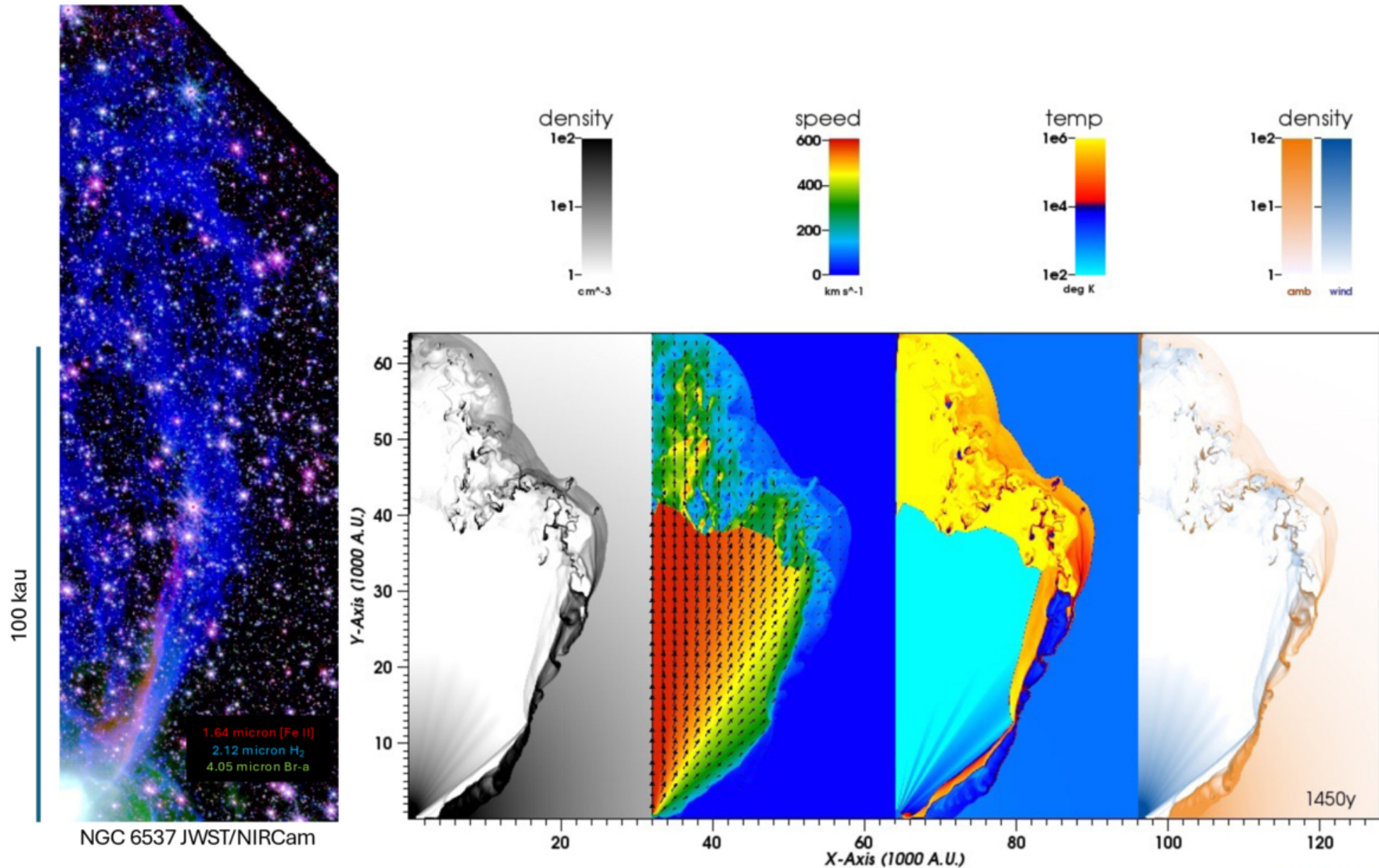
Figure 8. from Joel H. Kastner et al 2025 Astrophys. J. 993 doi:10.3847/1538-4357/ae0706 https://dx.doi.org/10.3847/1538-4357/ae0706 © 2025. The Author(s). Published by the American Astronomical Society.
