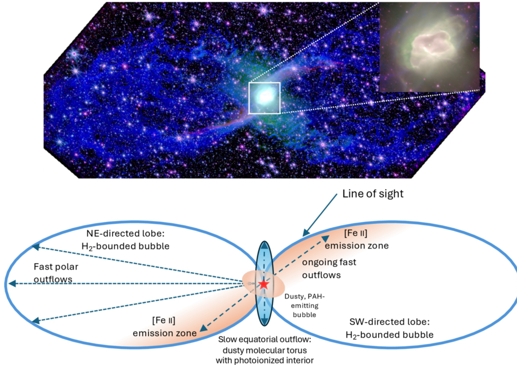
Figure 7. from Joel H. Kastner et al 2025 Astrophys. J. 993 doi:10.3847/1538-4357/ae0706 https://dx.doi.org/10.3847/1538-4357/ae0706 © 2025. The Author(s). Published by the American Astronomical Society.
