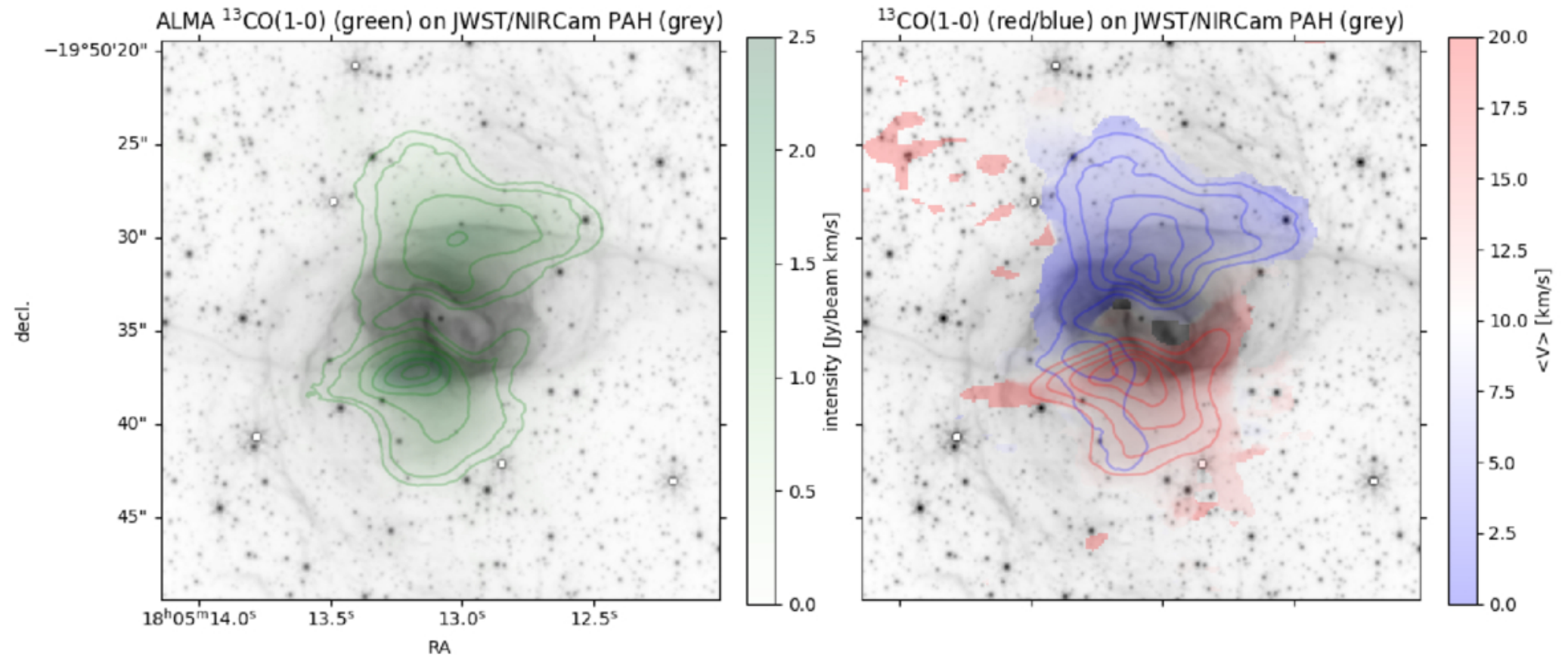
Figure 6. from Joel H. Kastner et al 2025 Astrophys. J. 993 doi:10.3847/1538-4357/ae0706 https://dx.doi.org/10.3847/1538-4357/ae0706 © 2025. The Author(s). Published by the American Astronomical Society.
