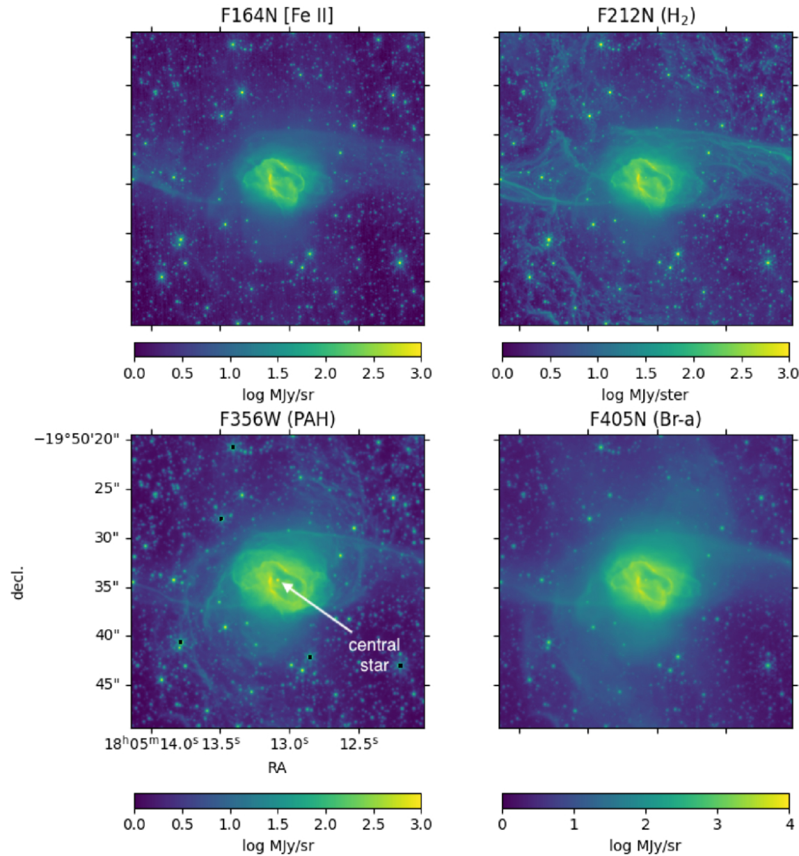
Figure 3. from Joel H. Kastner et al 2025 Astrophys. J. 993 doi:10.3847/1538-4357/ae0706 https://dx.doi.org/10.3847/1538-4357/ae0706 © 2025. The Author(s). Published by the American Astronomical Society.
