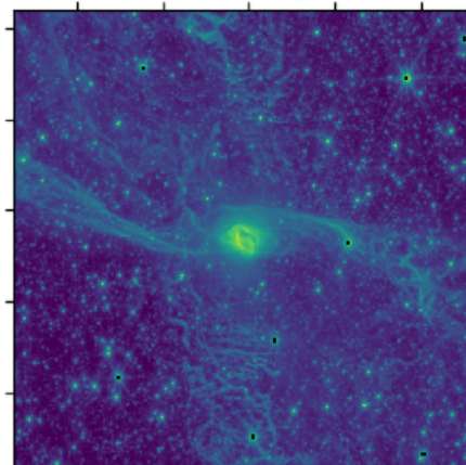
F212N (H 2 )
