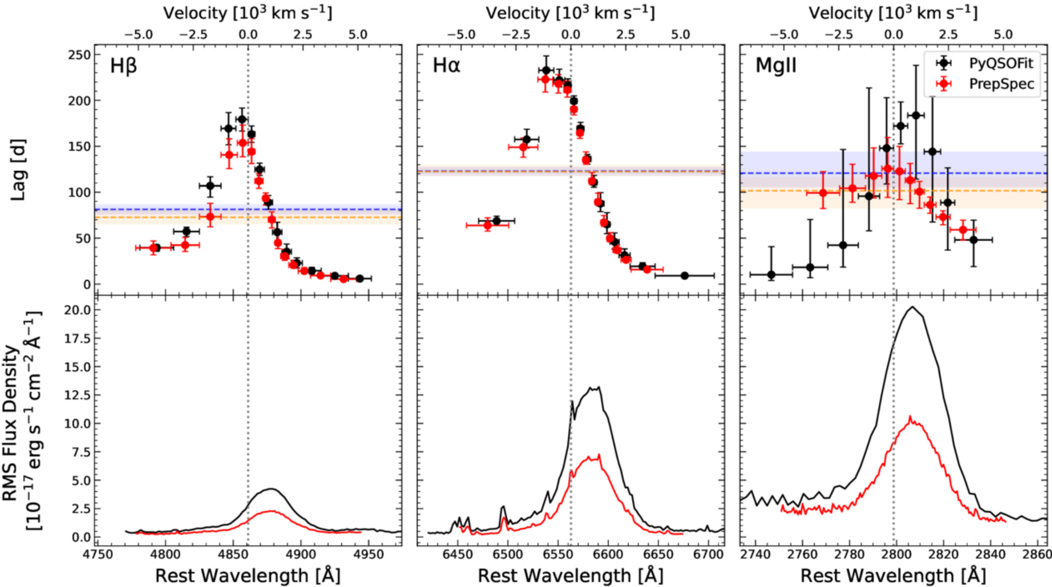
Figure 9. from Zachary Stone et al 2025 Astrophys. J. 991 doi:10.3847/1538-4357/adfd4c https://dx.doi.org/10.3847/1538-4357/adfd4c © 2025. The Author(s). Published by the American Astronomical Society.
