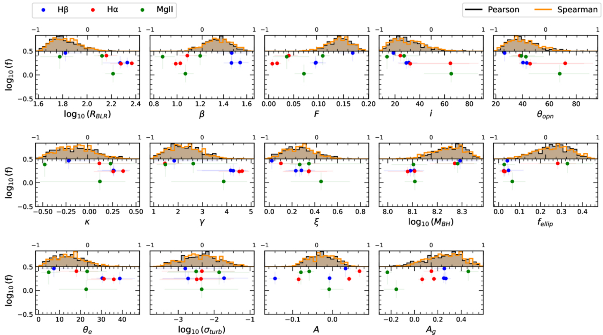
Figure 8. from Zachary Stone et al 2025 Astrophys. J. 991 doi:10.3847/1538-4357/adfd4c https://dx.doi.org/10.3847/1538-4357/adfd4c © 2025. The Author(s). Published by the American Astronomical Society.
