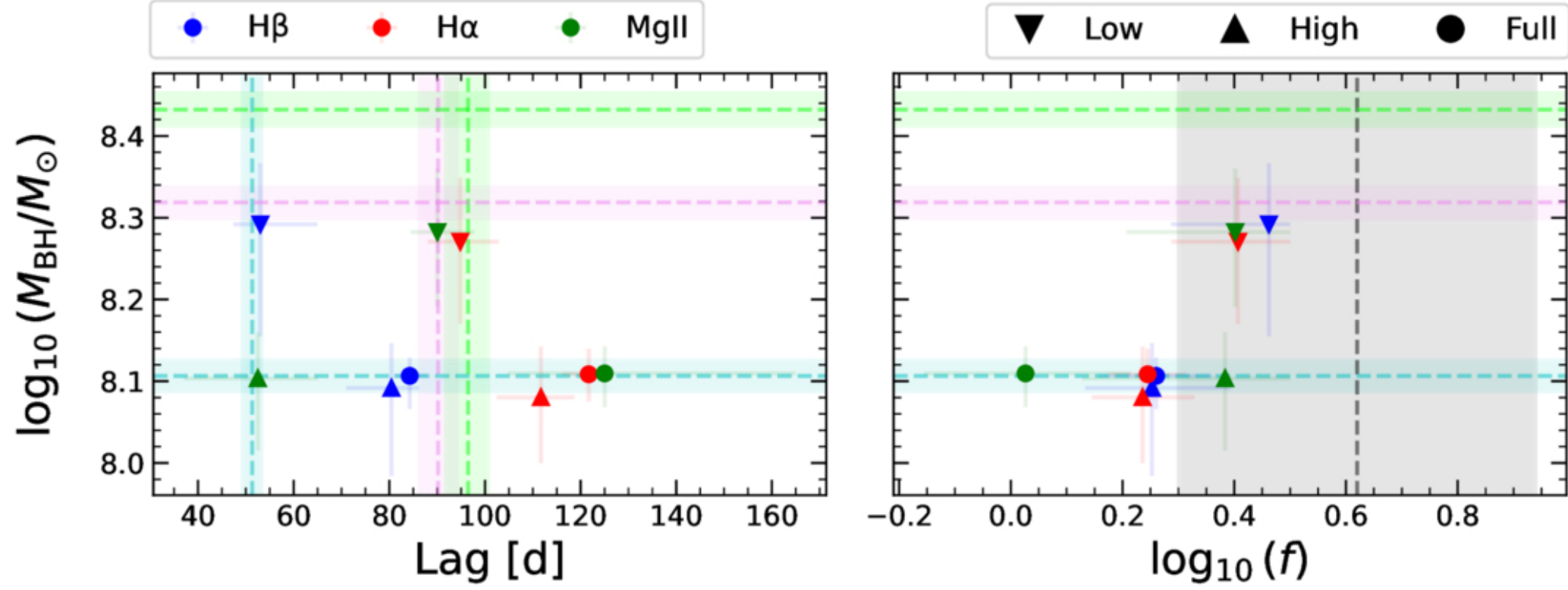
Figure 7. from Zachary Stone et al 2025 Astrophys. J. 991 doi:10.3847/1538-4357/adfd4c https://dx.doi.org/10.3847/1538-4357/adfd4c © 2025. The Author(s). Published by the American Astronomical Society.
