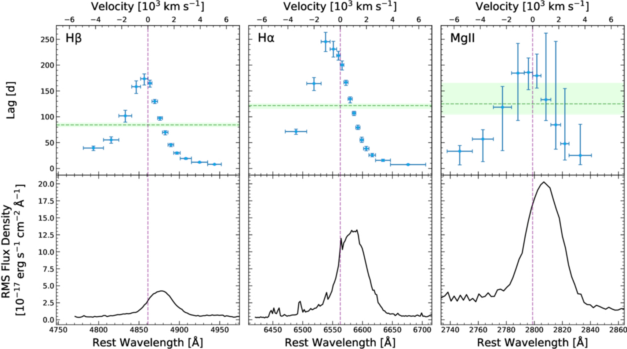
Figure 6. from Zachary Stone et al 2025 Astrophys. J. 991 doi:10.3847/1538-4357/adfd4c https://dx.doi.org/10.3847/1538-4357/adfd4c © 2025. The Author(s). Published by the American Astronomical Society.
