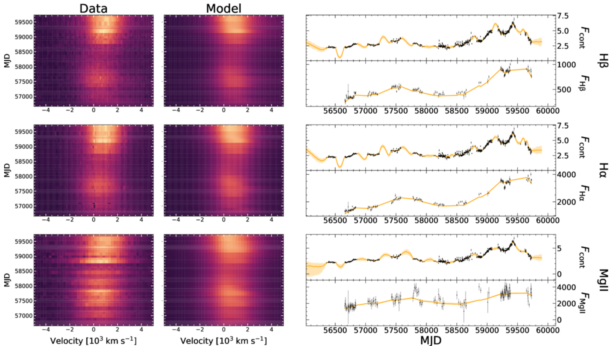
Figure 4. from Zachary Stone et al 2025 Astrophys. J. 991 doi:10.3847/1538-4357/adfd4c https://dx.doi.org/10.3847/1538-4357/adfd4c © 2025. The Author(s). Published by the American Astronomical Society.
