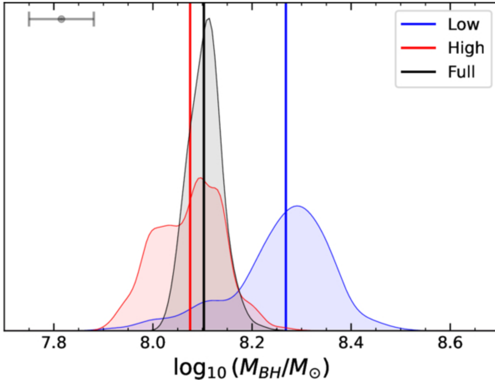
Figure 3. from Zachary Stone et al 2025 Astrophys. J. 991 doi:10.3847/1538-4357/adfd4c https://dx.doi.org/10.3847/1538-4357/adfd4c © 2025. The Author(s). Published by the American Astronomical Society.
