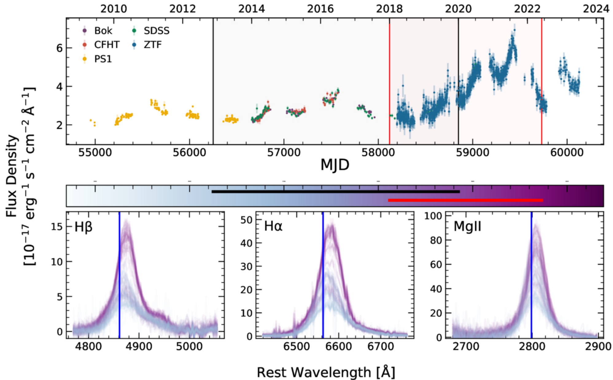
Figure 1. from Zachary Stone et al 2025 Astrophys. J. 991 doi:10.3847/1538-4357/adfd4c https://dx.doi.org/10.3847/1538-4357/adfd4c © 2025. The Author(s). Published by the American Astronomical Society.
