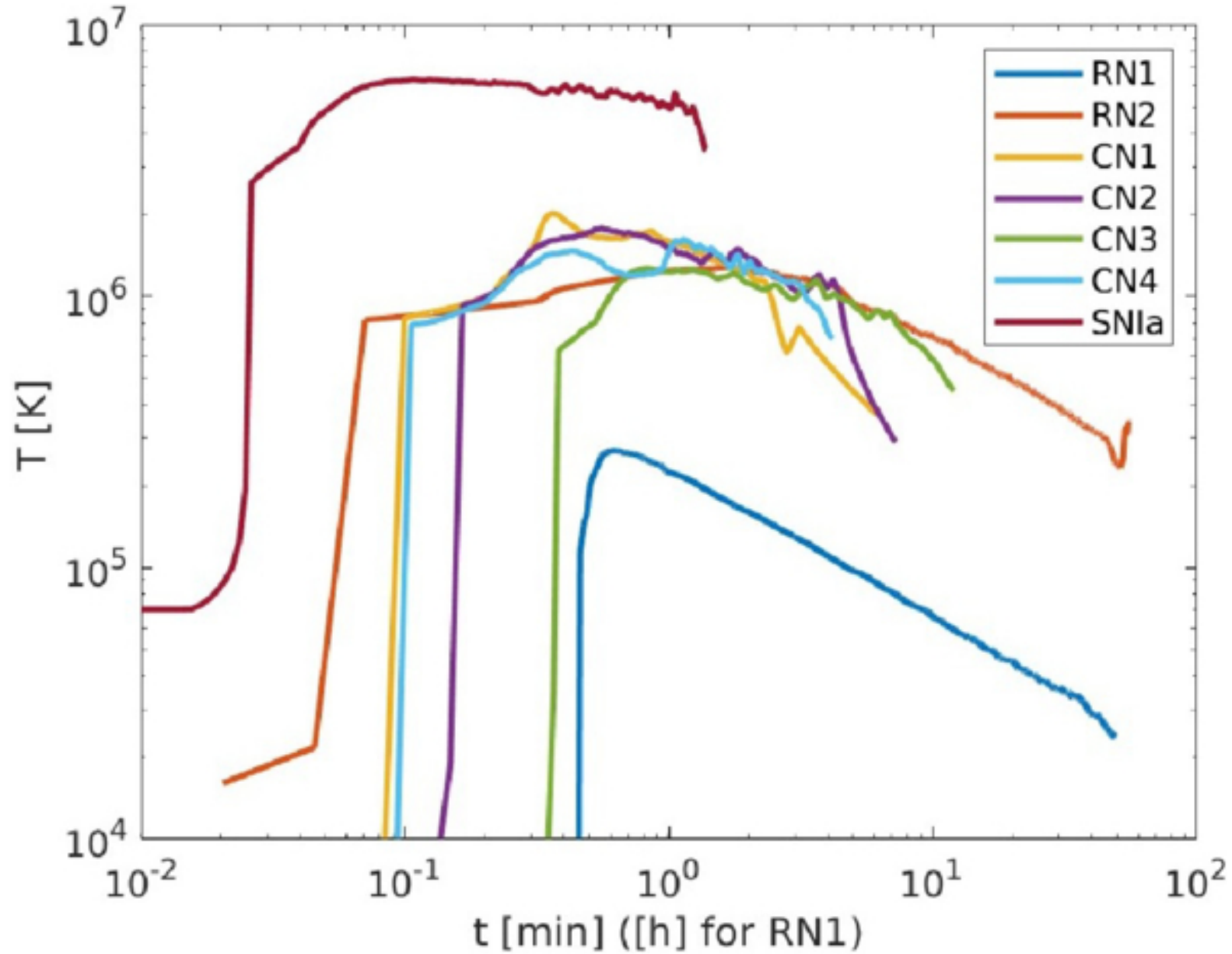
Figure 8. from Axel S. Lechuga et al 2025 Astrophys. J. 992 doi:10.3847/1538-4357/adfc5f https://dx.doi.org/10.3847/1538-4357/adfc5f © 2025. The Author(s). Published by the American Astronomical Society.
