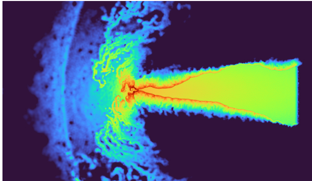
(a) RN1-Low: N = 500,000 particles
