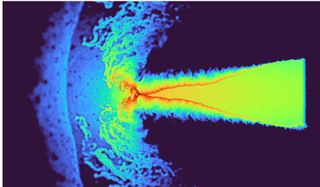
(b) RN1: N = 1,000,000 particles
