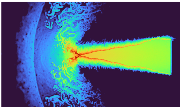
(c) RN1-High: N = 2,000,000 particles
