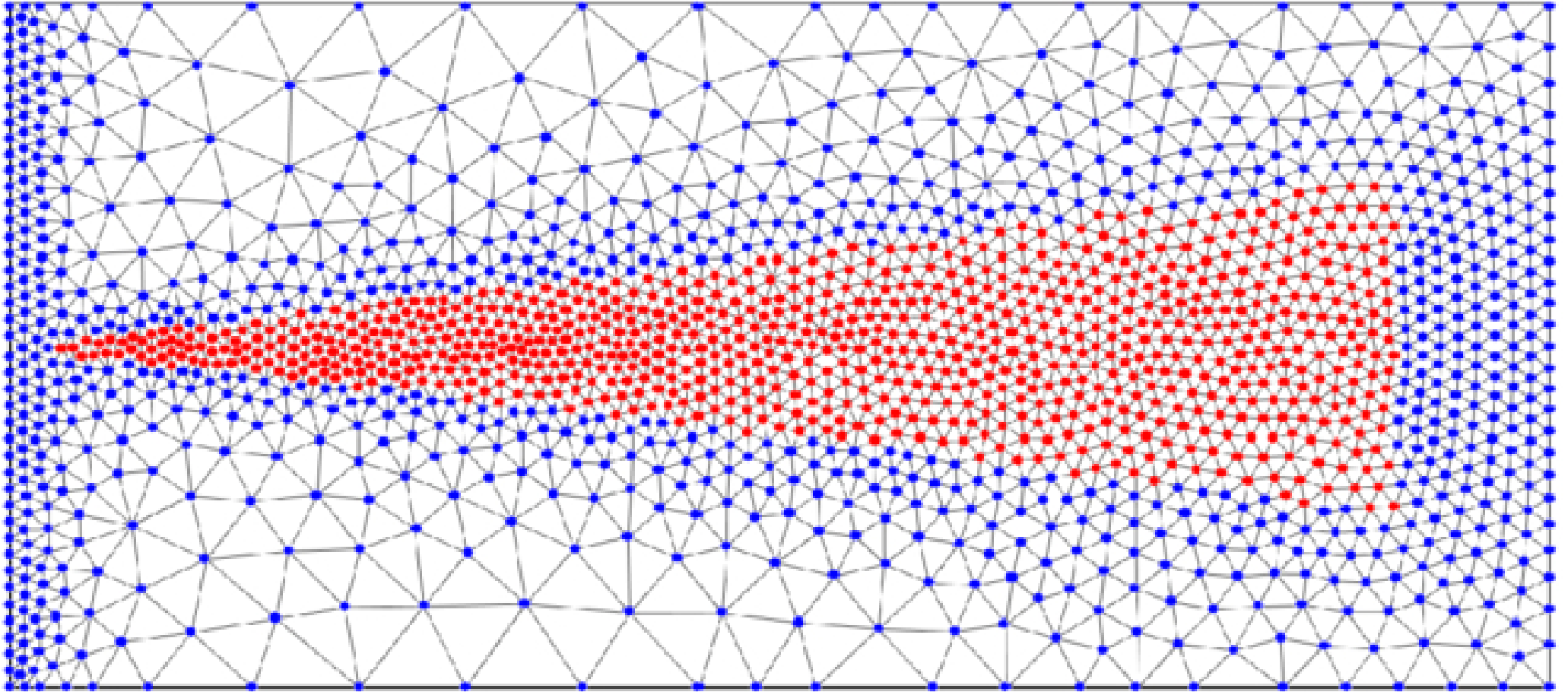
Figure 13. from Axel S. Lechuga et al 2025 Astrophys. J. 992 doi:10.3847/1538-4357/adfc5f https://dx.doi.org/10.3847/1538-4357/adfc5f © 2025. The Author(s). Published by the American Astronomical Society.
