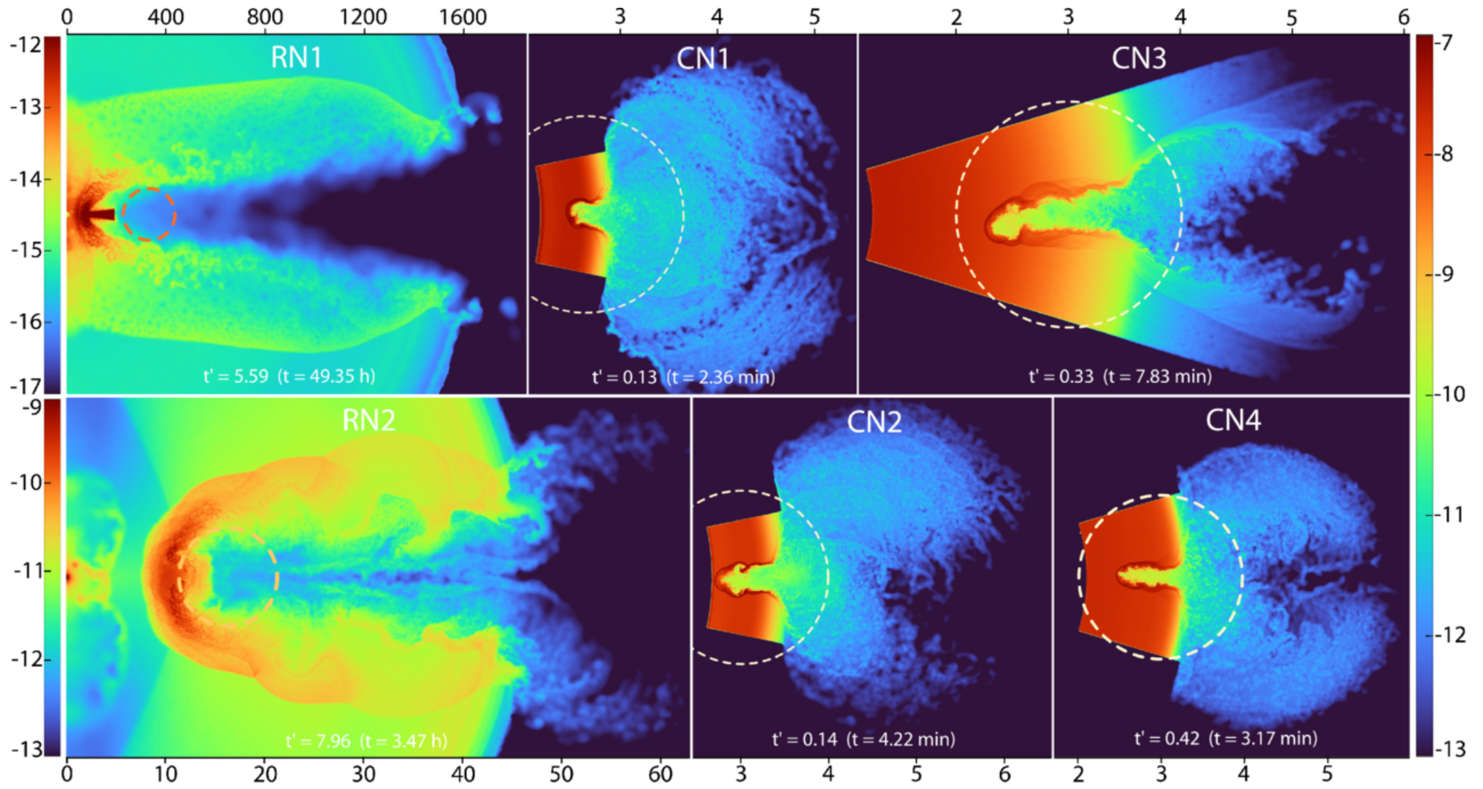
Figure 11. from Axel S. Lechuga et al 2025 Astrophys. J. 992 doi:10.3847/1538-4357/adfc5f https://dx.doi.org/10.3847/1538-4357/adfc5f © 2025. The Author(s). Published by the American Astronomical Society.
