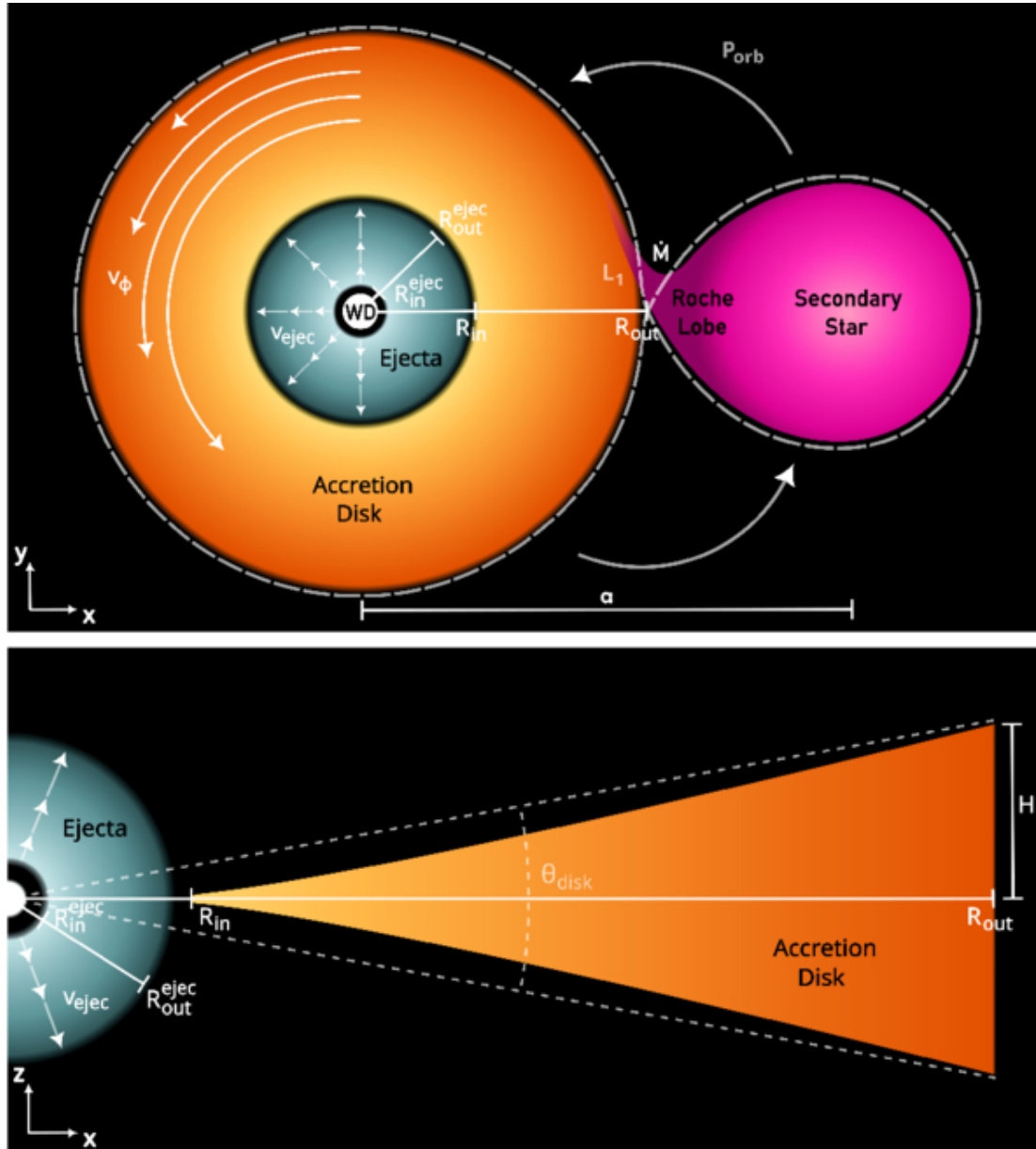
Figure 1. from Axel S. Lechuga et al 2025 Astrophys. J. 992 doi:10.3847/1538-4357/adfc5f https://dx.doi.org/10.3847/1538-4357/adfc5f © 2025. The Author(s). Published by the American Astronomical Society.
