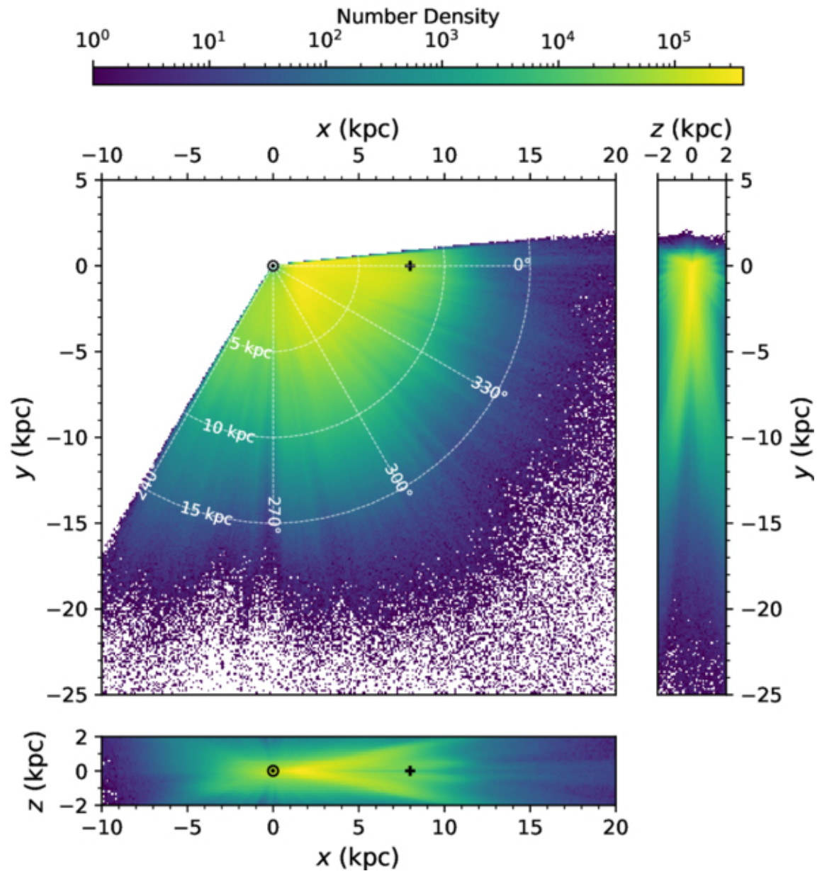
Figure 5. from Catherine Zucker et al 2025 Astrophys. J. 992 doi:10.3847/1538-4357/adf6e6 https://dx.doi.org/10.3847/1538-4357/adf6e6 © 2025. The Author(s). Published by the American Astronomical Society.
