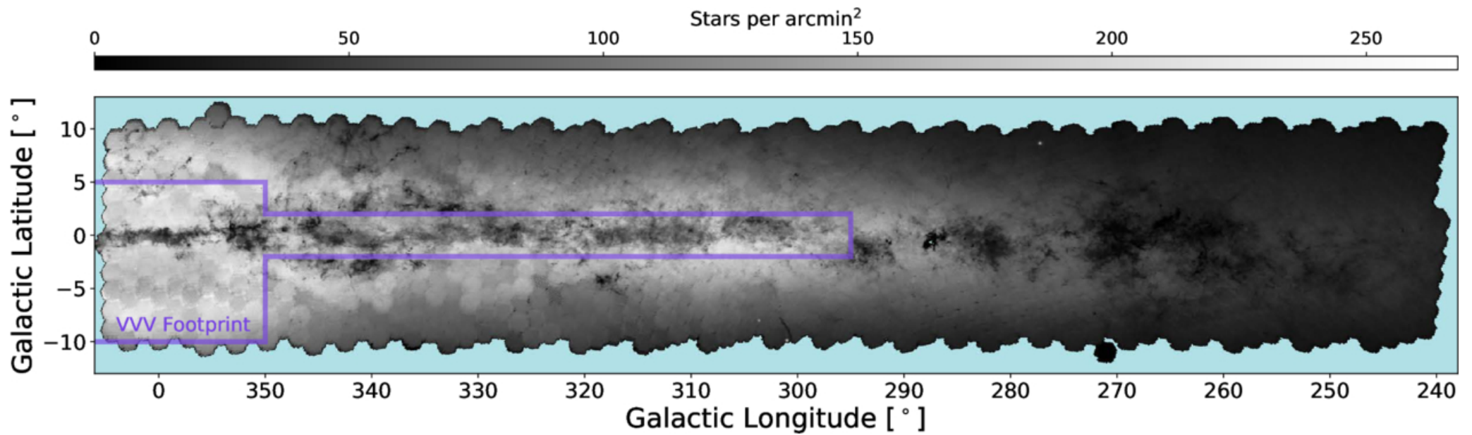
Figure 3. from Catherine Zucker et al 2025 Astrophys. J. 992 doi:10.3847/1538-4357/adf6e6 https://dx.doi.org/10.3847/1538-4357/adf6e6 © 2025. The Author(s). Published by the American Astronomical Society.
