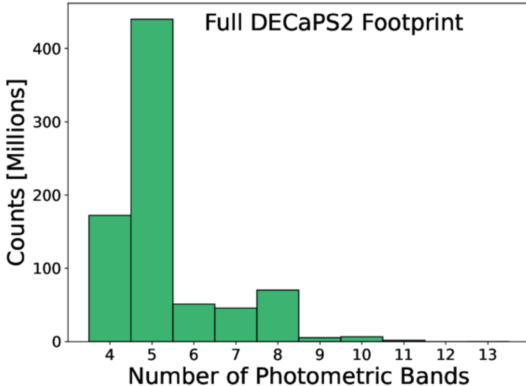
Figure 2. from Catherine Zucker et al 2025 Astrophys. J. 992 doi:10.3847/1538-4357/adfbe6 https://dx.doi.org/10.3847/1538-4357/adfbe6 © 2025. The Author(s). Published by the American Astronomical Society.
