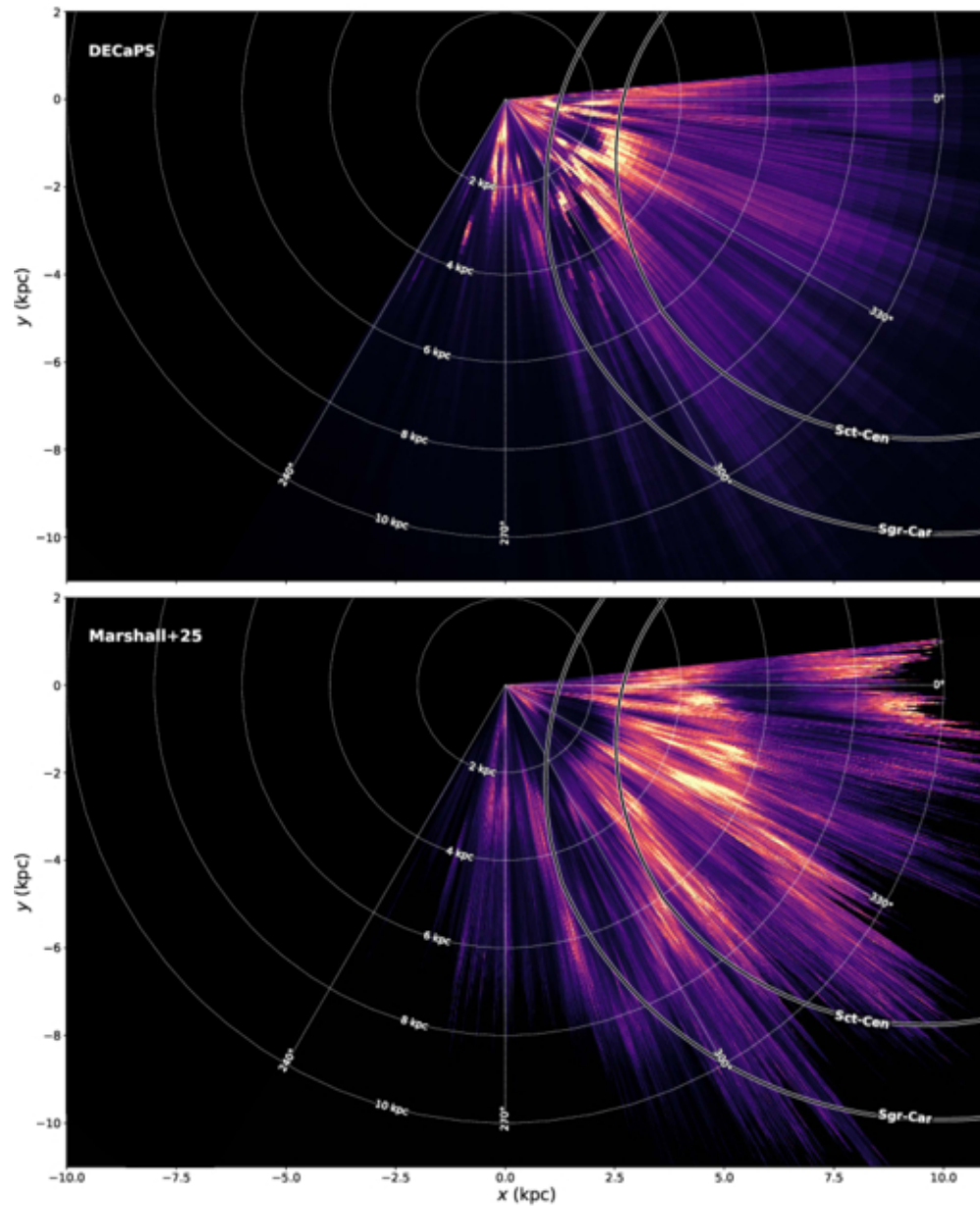
Figure 14. from Catherine Zucker et al 2025 Astrophys. J. 992 doi:10.3847/1538-4357/adfbe6 https://dx.doi.org/10.3847/1538-4357/adfbe6 © 2025. The Author(s). Published by the American Astronomical Society.
