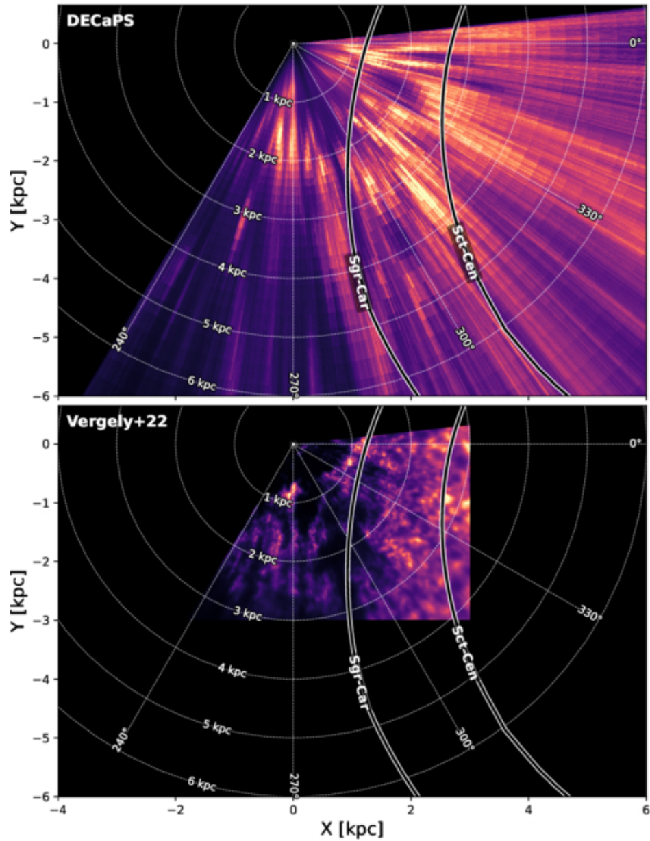
Figure 11. from Catherine Zucker et al 2025 Astrophys. J. 992 doi:10.3847/1538-4357/adf6e6 https://dx.doi.org/10.3847/1538-4357/adf6e6 © 2025. The Author(s). Published by the American Astronomical Society.
