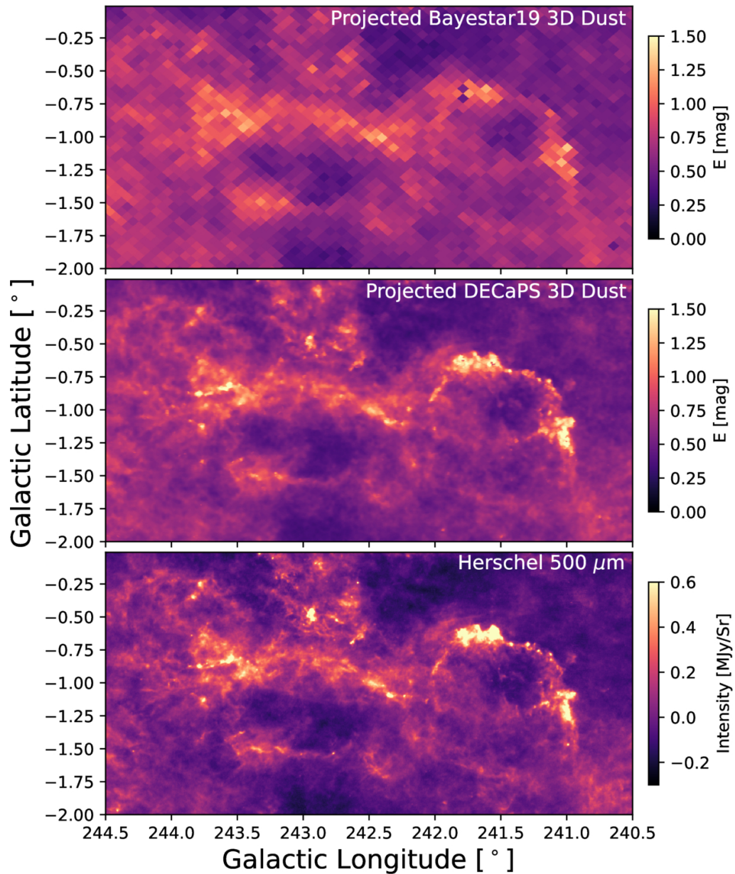
Figure 10. from Catherine Zucker et al 2025 Astrophys. J. 992 doi:10.3847/1538-4357/adf6e6 https://dx.doi.org/10.3847/1538-4357/adf6e6 © 2025. The Author(s). Published by the American Astronomical Society.
