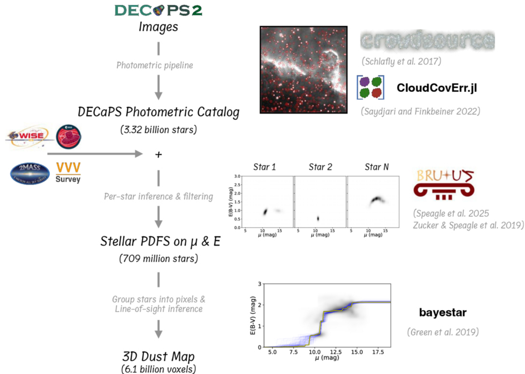
Figure 1. from Catherine Zucker et al 2025 Astrophys. J. 992 doi:10.3847/1538-4357/adfbe6 https://dx.doi.org/10.3847/1538-4357/adfbe6 © 2025. The Author(s). Published by the American Astronomical Society.
