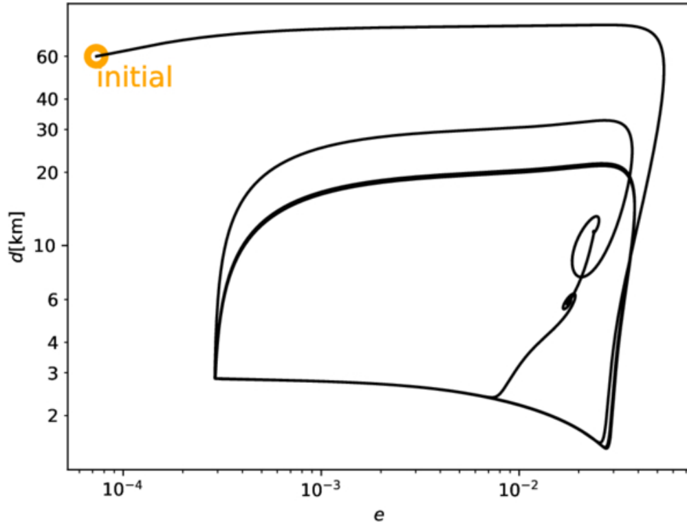
Figure 9. from Peter Goldreich et al 2025 Astrophys. J. 992 doi:10.3847/1538-4357/adf8e7 https://dx.doi.org/10.3847/1538-4357/adf8e7 © 2025. The Author(s). Published by the American Astronomical Society.
