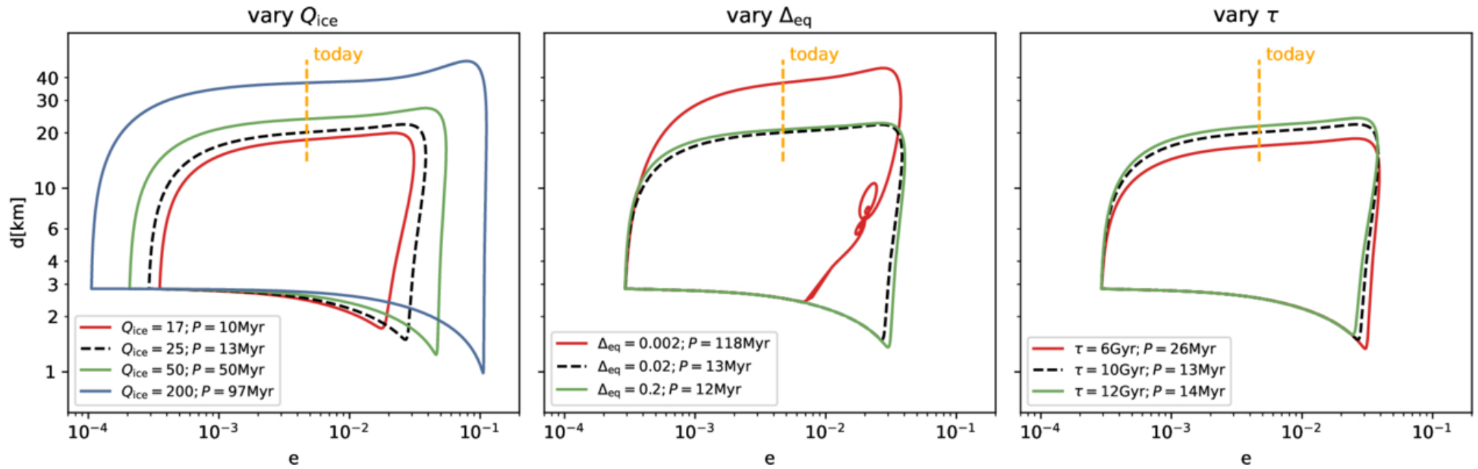
Figure 8. from Peter Goldreich et al 2025 Astrophys. J. 992 doi:10.3847/1538-4357/adf8e7 https://dx.doi.org/10.3847/1538-4357/adf8e7 © 2025. The Author(s). Published by the American Astronomical Society.
