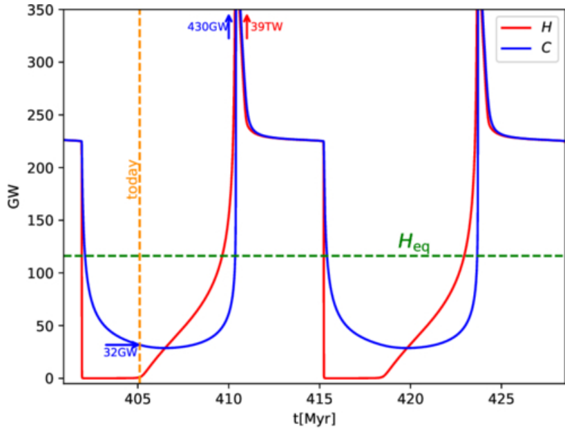
Figure 6. from Peter Goldreich et al 2025 Astrophys. J. 992 doi:10.3847/1538-4357/adf8e7 https://dx.doi.org/10.3847/1538-4357/adf8e7 © 2025. The Author(s). Published by the American Astronomical Society.
