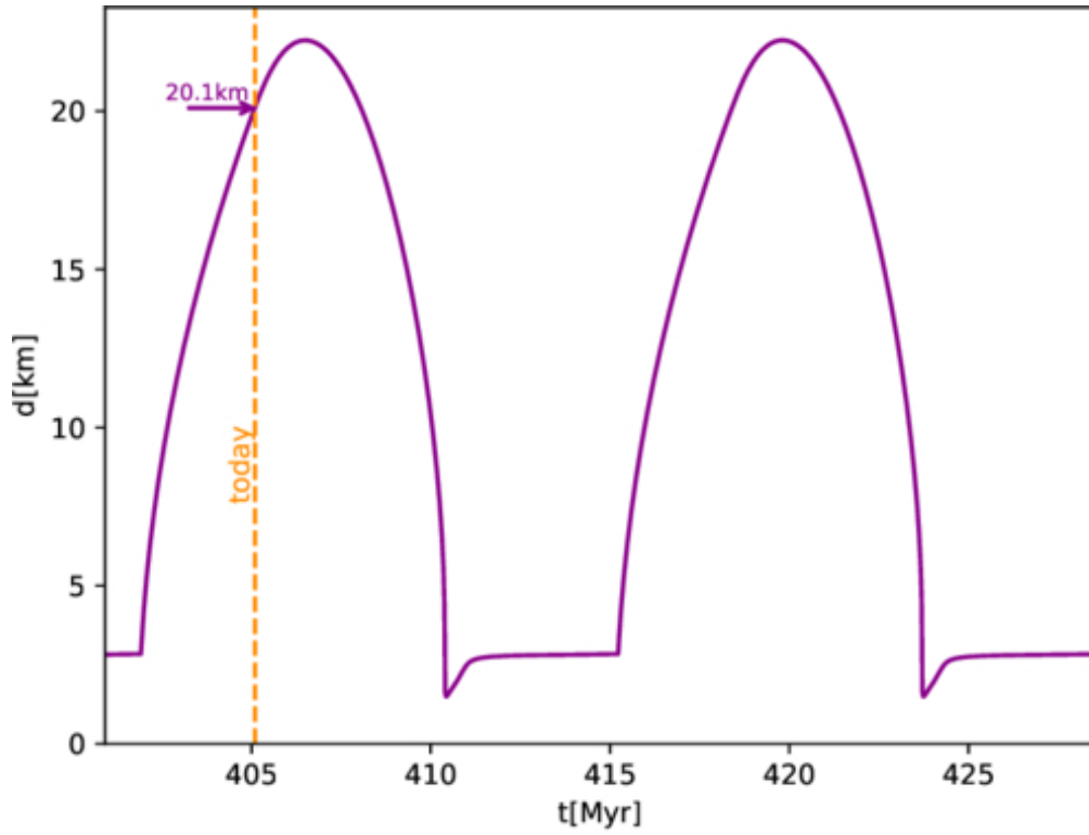
Figure 5. from Peter Goldreich et al 2025 Astrophys. J. 992 doi:10.3847/1538-4357/adf8e7 https://dx.doi.org/10.3847/1538-4357/adf8e7 © 2025. The Author(s). Published by the American Astronomical Society.
