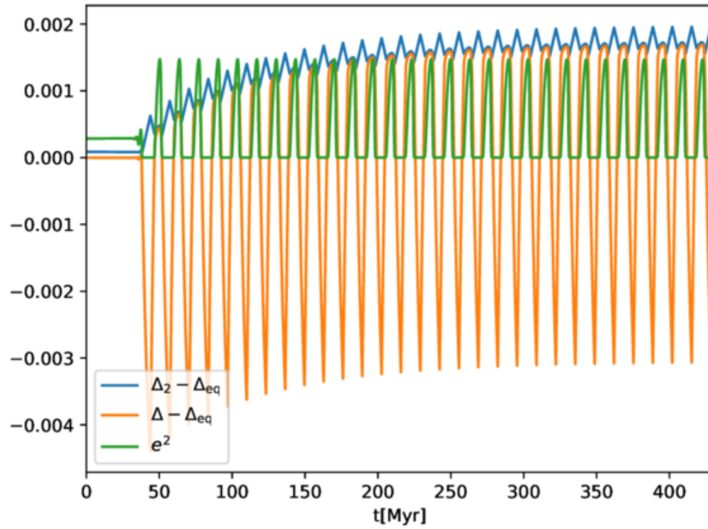
Figure 4. from Peter Goldreich et al 2025 Astrophys. J. 992 doi:10.3847/1538-4357/adf8e7 https://dx.doi.org/10.3847/1538-4357/adf8e7 © 2025. The Author(s). Published by the American Astronomical Society.
