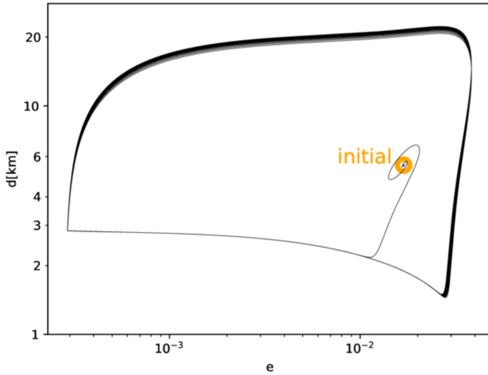
Figure 3. from Peter Goldreich et al 2025 Astrophys. J. 992 doi:10.3847/1538-4357/adf8e7 https://dx.doi.org/10.3847/1538-4357/adf8e7 © 2025. The Author(s). Published by the American Astronomical Society.
