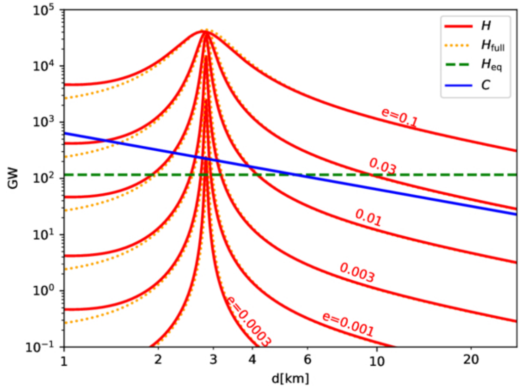
Figure 2. from Peter Goldreich et al 2025 Astrophys. J. 992 doi:10.3847/1538-4357/adf8e7 https://dx.doi.org/10.3847/1538-4357/adf8e7 © 2025. The Author(s). Published by the American Astronomical Society.
