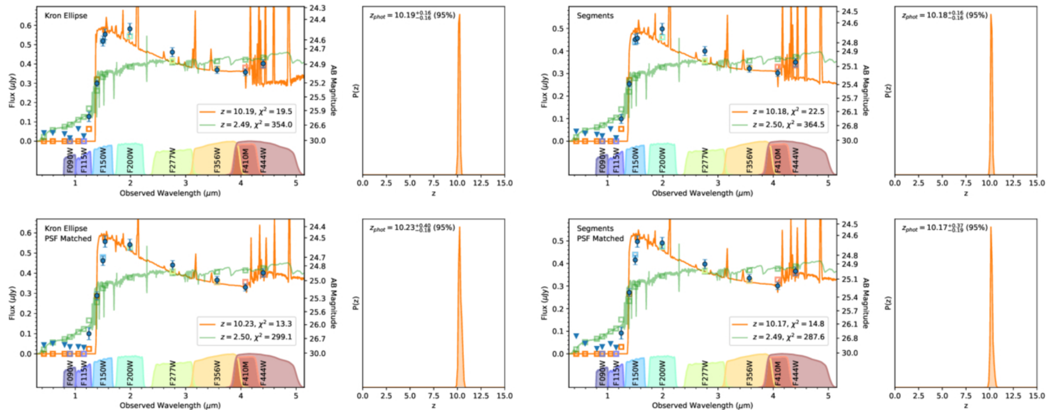
Figure 7. from Larry D. Bradley et al 2025 Astrophys. J. 991 doi:10.3847/1538-4357/adf638 https://dx.doi.org/10.3847/1538-4357/adf638 © 2025. The Author(s). Published by the American Astronomical Society.
