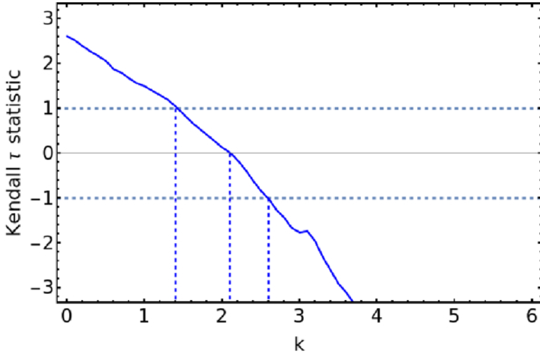
Figure 2. from Nikita S. Khatiya et al 2025 Astrophys. J. 990 doi:10.3847/1538-4357/adf219 https://dx.doi.org/10.3847/1538-4357/adf219 © 2025. The Author(s). Published by the American Astronomical Society.
