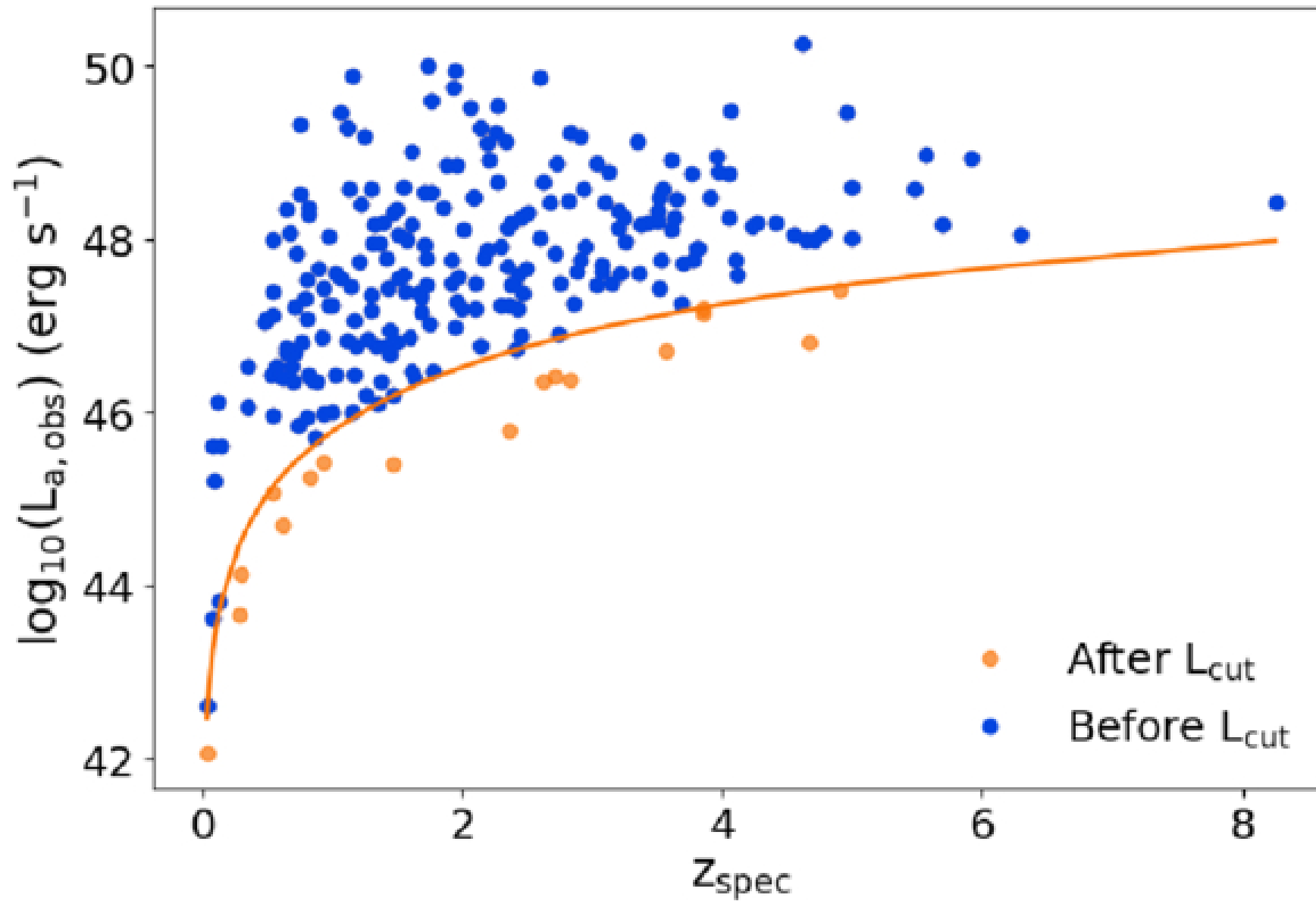
Figure 1. from Nikita S. Khatiya et al 2025 Astrophys. J. 990 doi:10.3847/1538-4357/adf219 https://dx.doi.org/10.3847/1538-4357/adf219 © 2025. The Author(s). Published by the American Astronomical Society.
