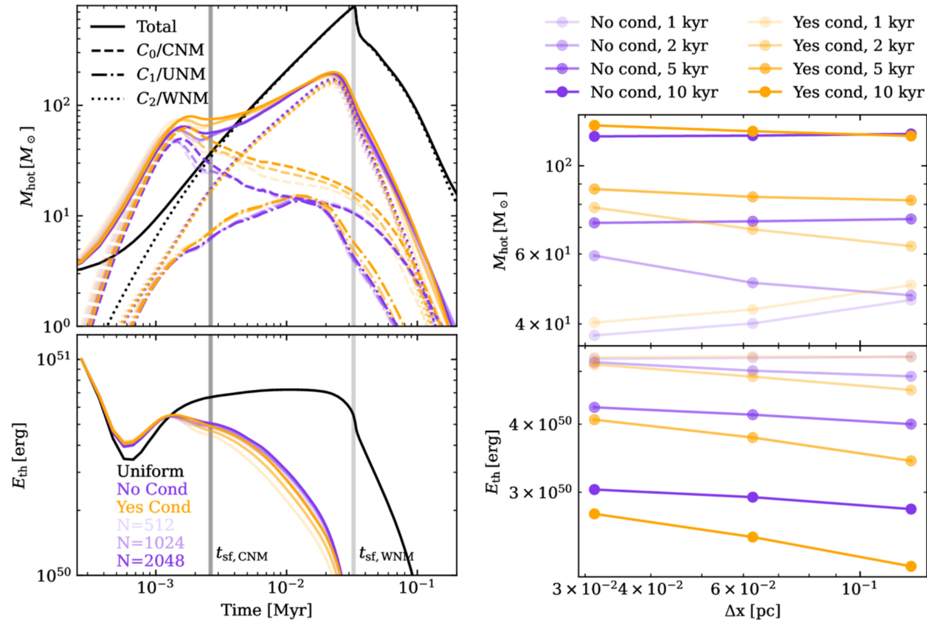
Figure 8. from Minghao Guo et al 2025 Astrophys. J. 990 doi:10.3847/1538-4357/adeb85 https://dx.doi.org/10.3847/1538-4357/adeb85 © 2025. The Author(s). Published by the American Astronomical Society.
