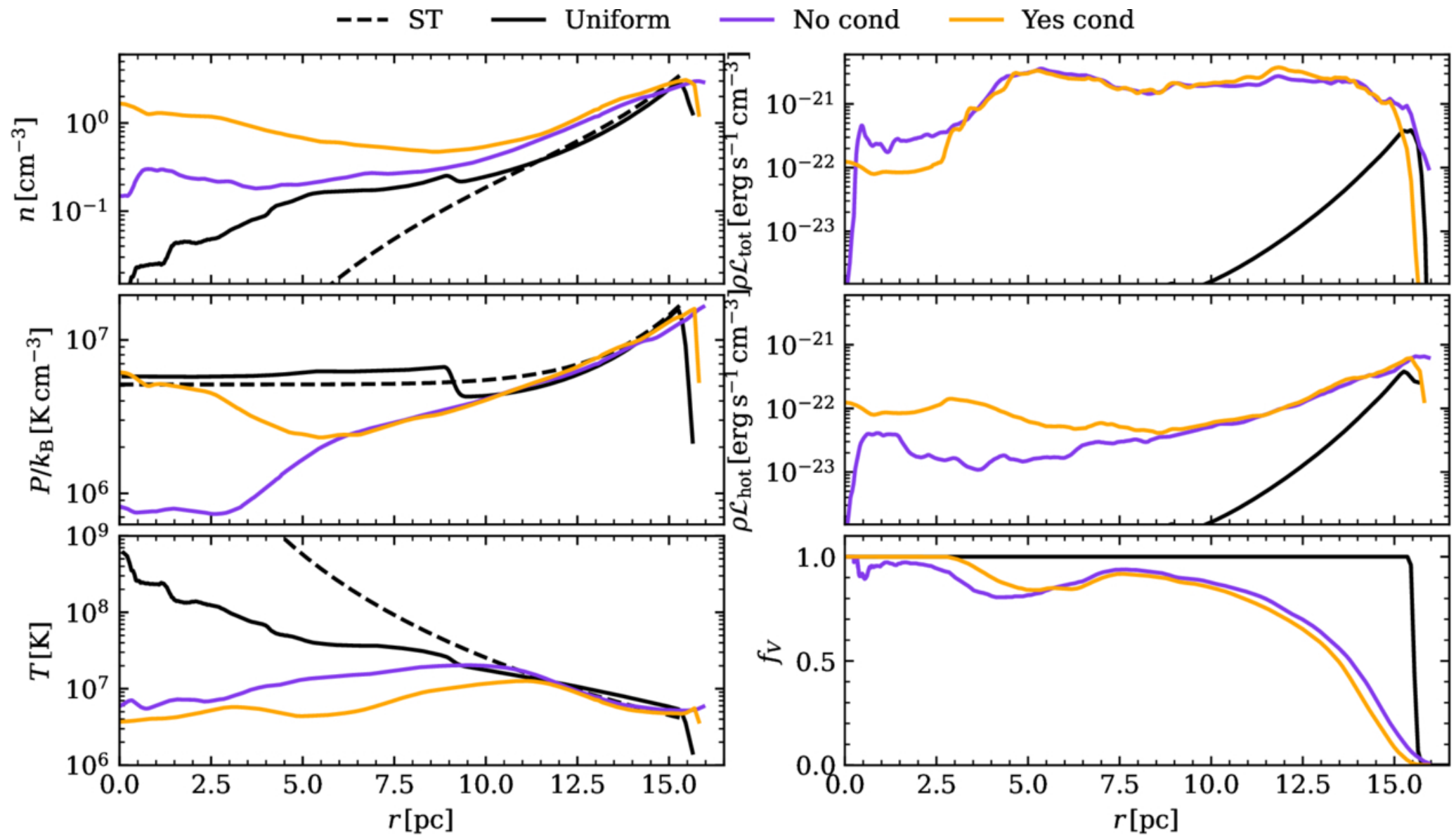
Figure 6. from Minghao Guo et al 2025 Astrophys. J. 990 doi:10.3847/1538-4357/adeb85 https://dx.doi.org/10.3847/1538-4357/adeb85 © 2025. The Author(s). Published by the American Astronomical Society.
