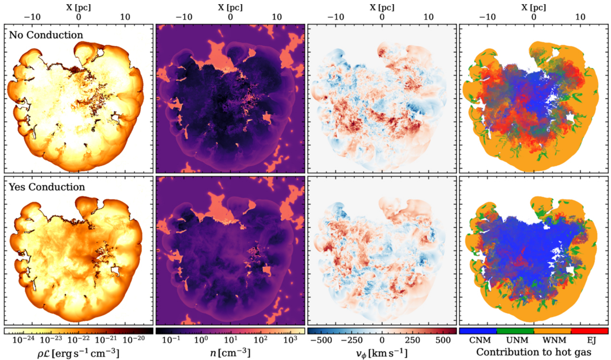
Figure 5. from Minghao Guo et al 2025 Astrophys. J. 990 doi:10.3847/1538-4357/adeb85 https://dx.doi.org/10.3847/1538-4357/adeb85 © 2025. The Author(s). Published by the American Astronomical Society.
