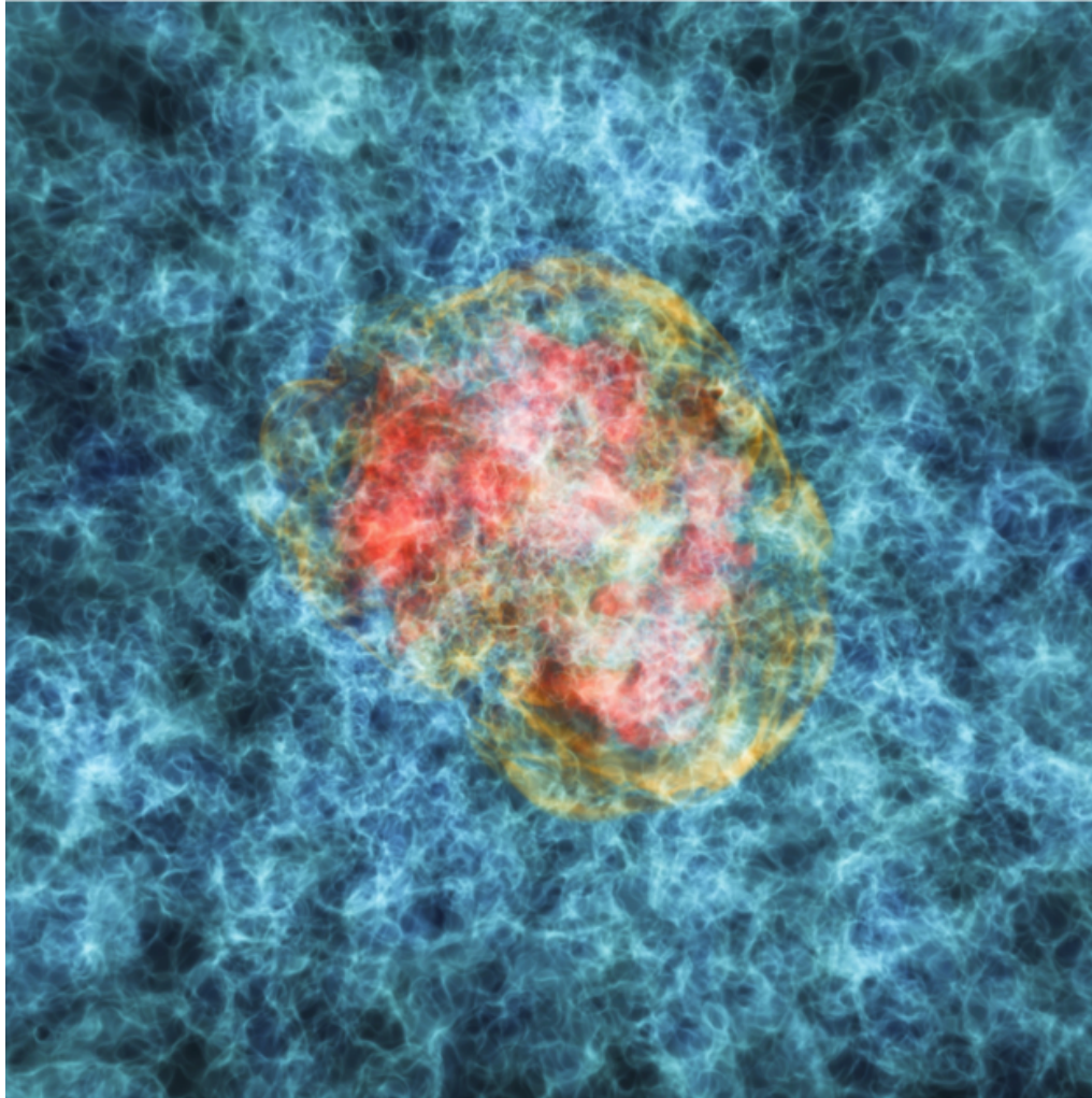
Figure 2. from Minghao Guo et al 2025 Astrophys. J. 990 doi:10.3847/1538-4357/adeb85 https://dx.doi.org/10.3847/1538-4357/adeb85 © 2025. The Author(s). Published by the American Astronomical Society.
