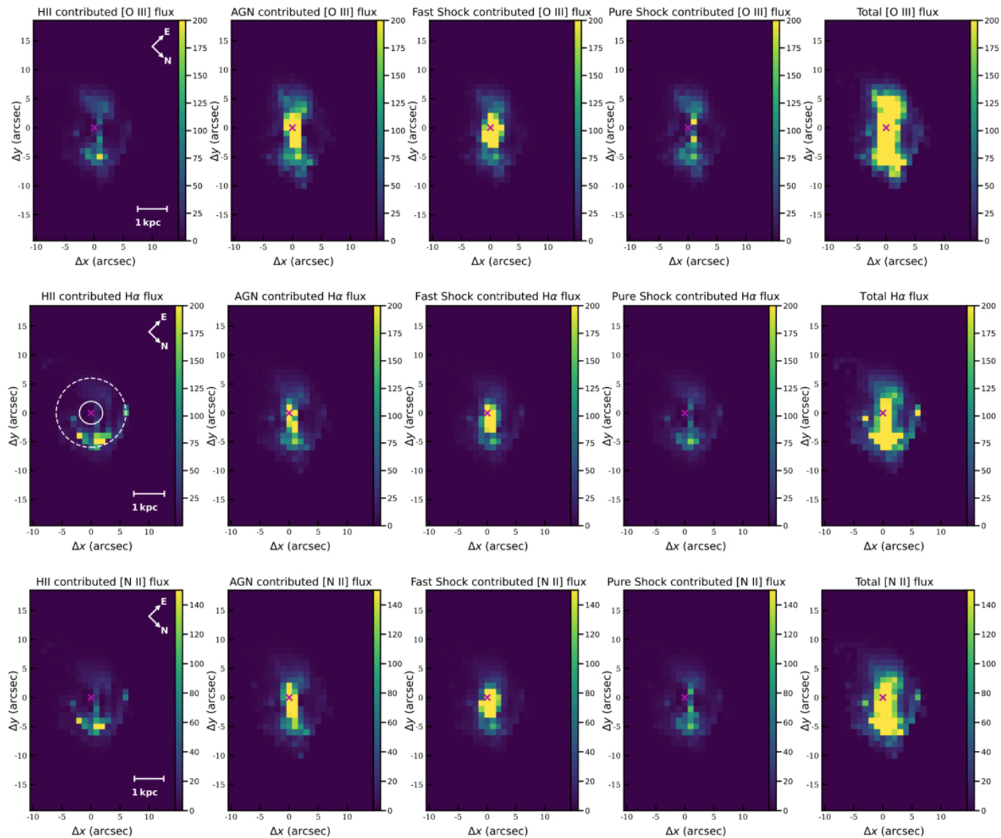
Figure 7. from Peixin Zhu et al 2025 Astrophys. J. 988 doi:10.3847/1538-4357/ade78f https://dx.doi.org/10.3847/1538-4357/ade78f © 2025. The Author(s). Published by the American Astronomical Society.
