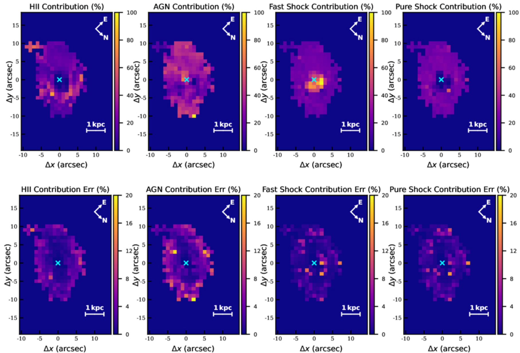
Figure 6. from Peixin Zhu et al 2025 Astrophys. J. 988 doi:10.3847/1538-4357/ade78f https://dx.doi.org/10.3847/1538-4357/ade78f © 2025. The Author(s). Published by the American Astronomical Society.
