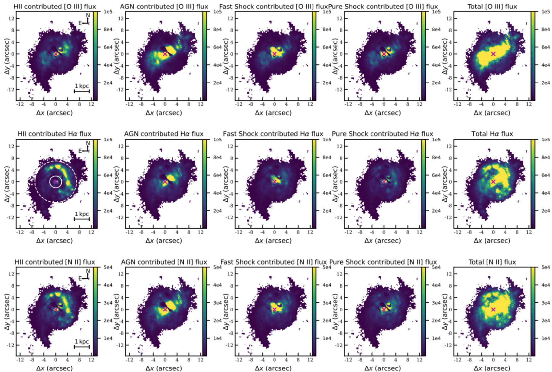
Figure 4. from Peixin Zhu et al 2025 Astrophys. J. 988 doi:10.3847/1538-4357/ade78f https://dx.doi.org/10.3847/1538-4357/ade78f © 2025. The Author(s). Published by the American Astronomical Society.
