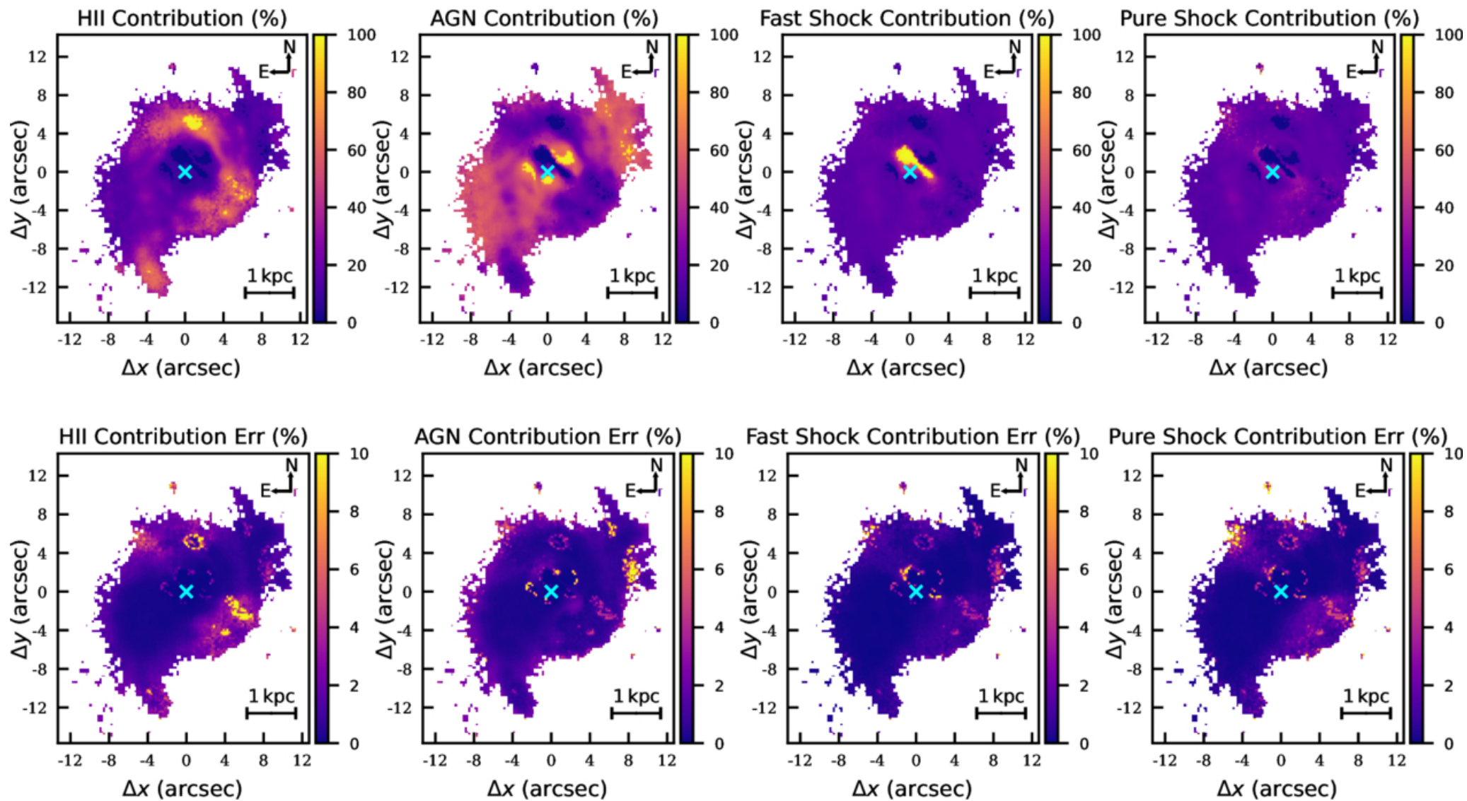
Figure 3. from Peixin Zhu et al 2025 Astrophys. J. 988 doi:10.3847/1538-4357/ade78f https://dx.doi.org/10.3847/1538-4357/ade78f © 2025. The Author(s). Published by the American Astronomical Society.
