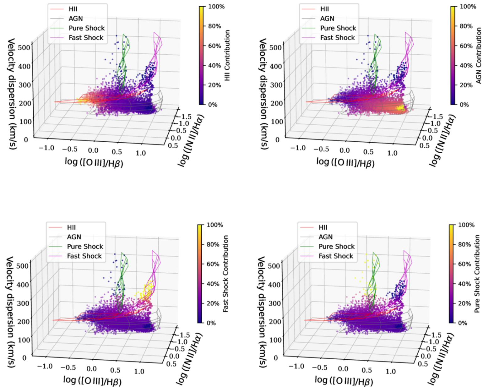
Figure 2. from Peixin Zhu et al 2025 Astrophys. J. 988 doi:10.3847/1538-4357/ade78f https://dx.doi.org/10.3847/1538-4357/ade78f © 2025. The Author(s). Published by the American Astronomical Society.
