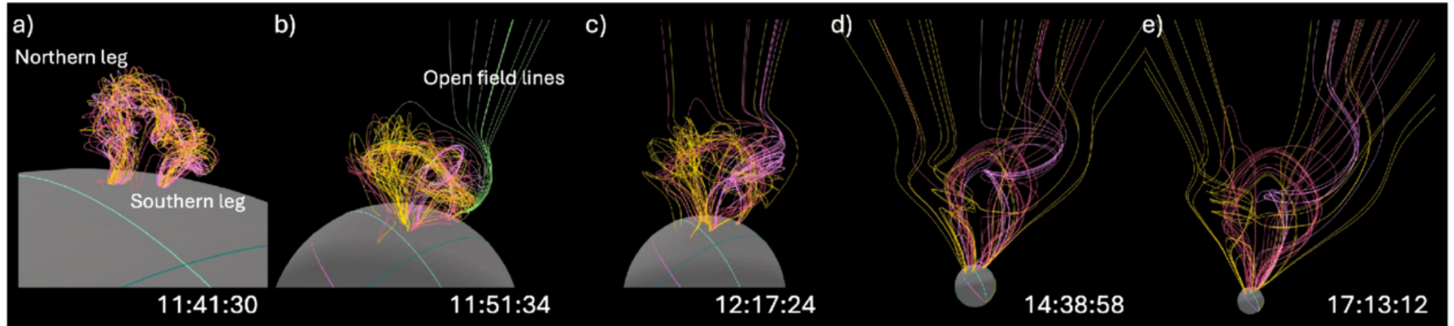
Figure 4. from Cecilia Mac Cormack et al 2025 Astrophys. J. 988 doi:10.3847/1538-4357/ade311 https://dx.doi.org/10.3847/1538-4357/ade311 © 2025. The Author(s). Published by the American Astronomical Society.
