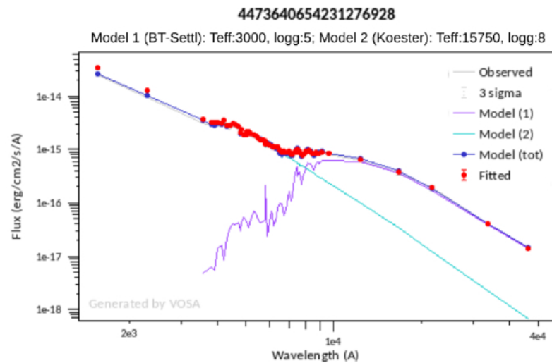
(b) Photometric points found by VOSA for the cool WDMS prototype and fitted to a binary SED
