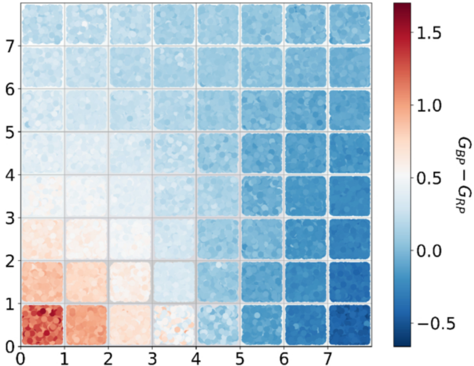
Figure 5. from Xabier Pérez-Couto et al 2025 Astrophys. J. 988 doi:10.3847/1538-4357/addfd7 https://dx.doi.org/10.3847/1538-4357/addfd7 © 2025. The Author(s). Published by the American Astronomical Society.
