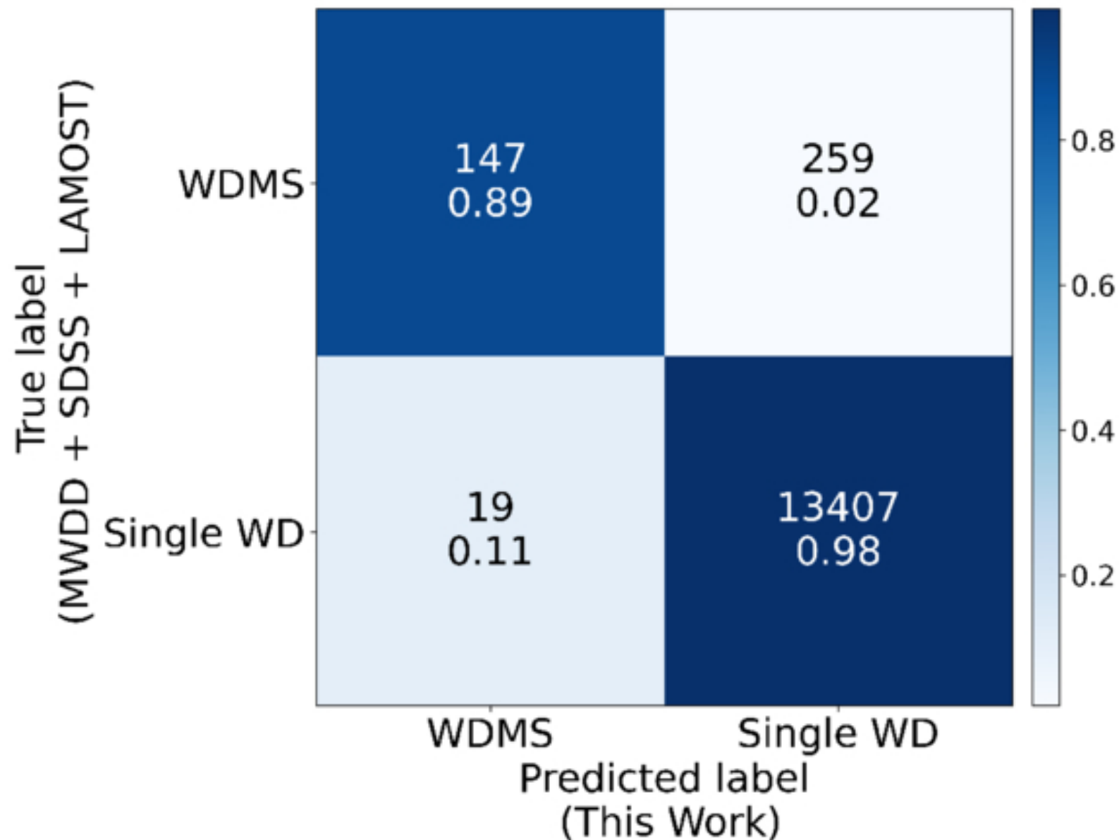
Figure 4. from Xabier Pérez-Couto et al 2025 Astrophys. J. 988 doi:10.3847/1538-4357/addfd7 https://dx.doi.org/10.3847/1538-4357/addfd7 © 2025. The Author(s). Published by the American Astronomical Society.
