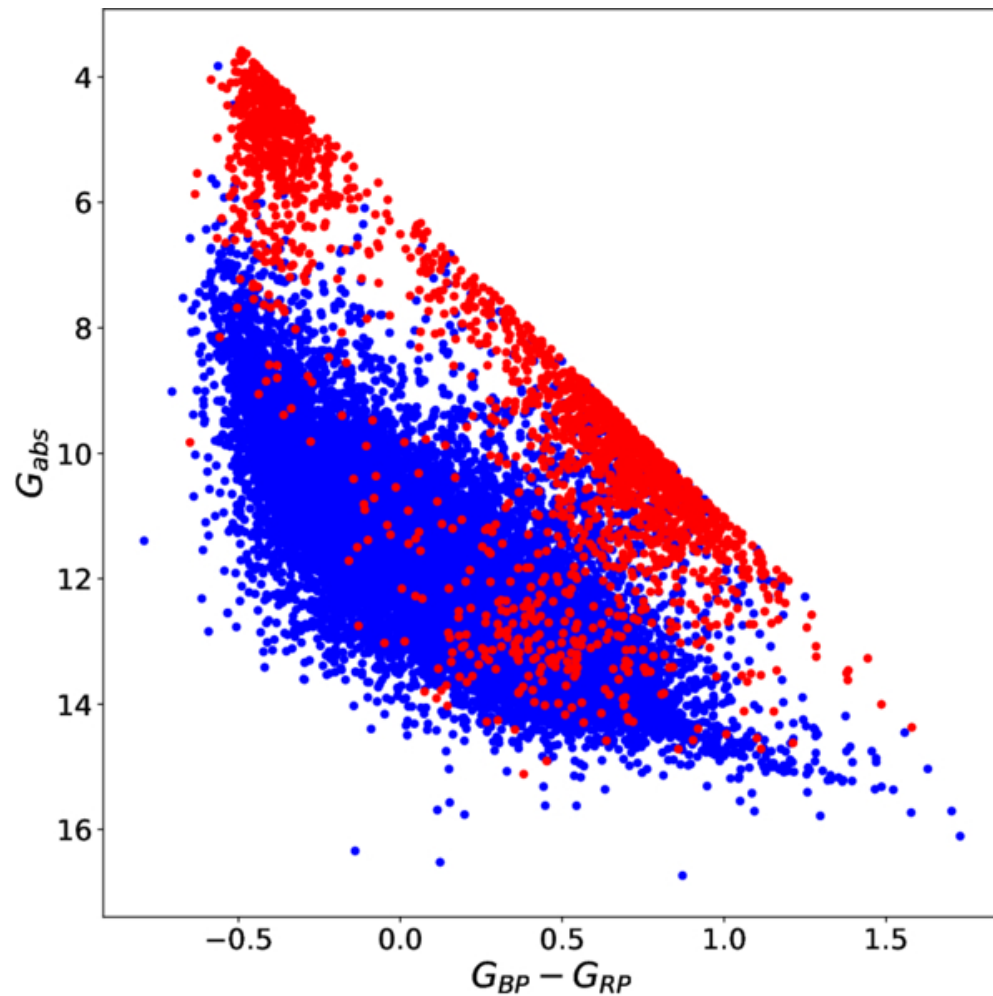
Figure 1. from Xabier Pérez-Couto et al 2025 Astrophys. J. 988 doi:10.3847/1538-4357/addfd7 https://dx.doi.org/10.3847/1538-4357/addfd7 © 2025. The Author(s). Published by the American Astronomical Society.
