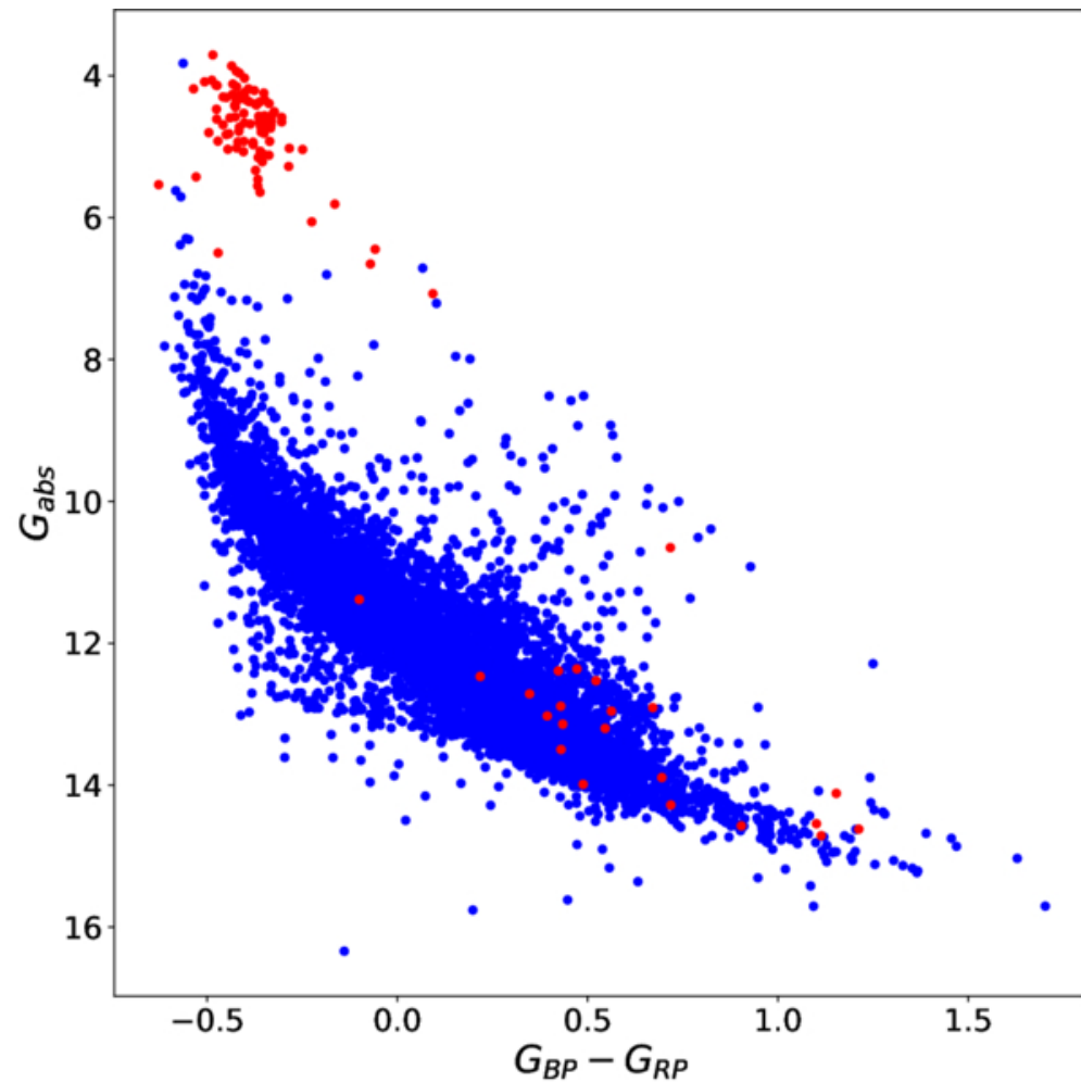
(b) \bar{\omega}/\sigma_{\bar{\omega}} > 10
